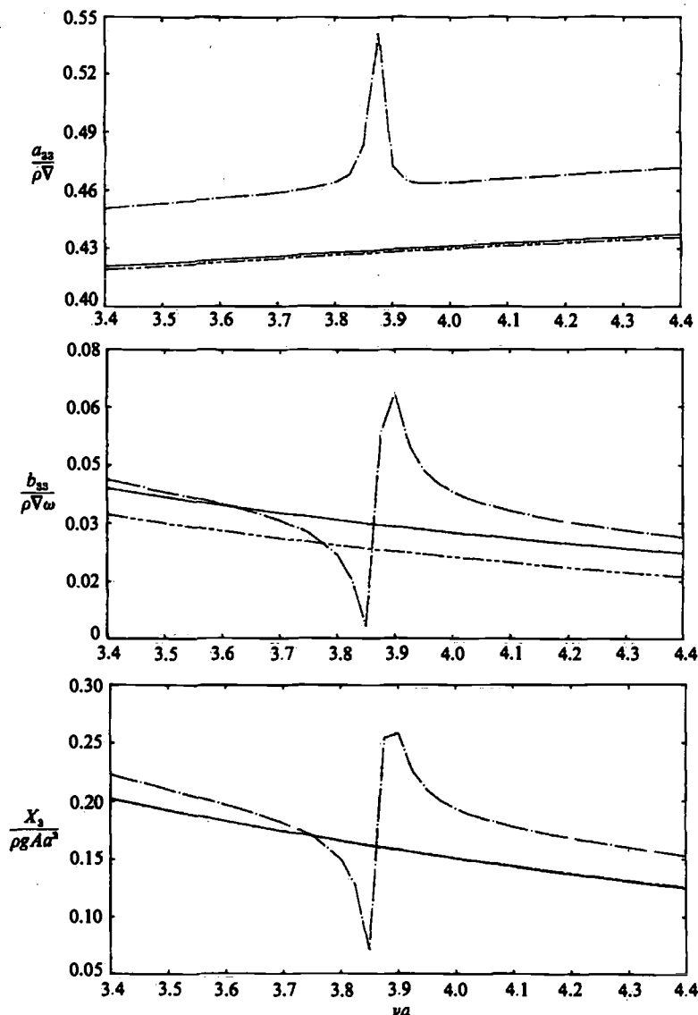
FIGURE 7. Heave added-mass and damping coefficients and modulus of the exciting force on the sphere near the second Neumann irregular frequency, as functions of \nu a : ----, \beta = 0 ; —, \beta = 0.11 ; - · -, \beta = \infty .
