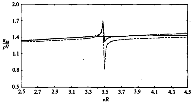
FIGURE 12. Heave added mass on the cylinder near the common irregular frequency of equations (2.8) and (3.15), as functions of \nu R : - - - - , \beta = 0 ; — , \beta = 0.15 ; — · — , \beta = \infty .
