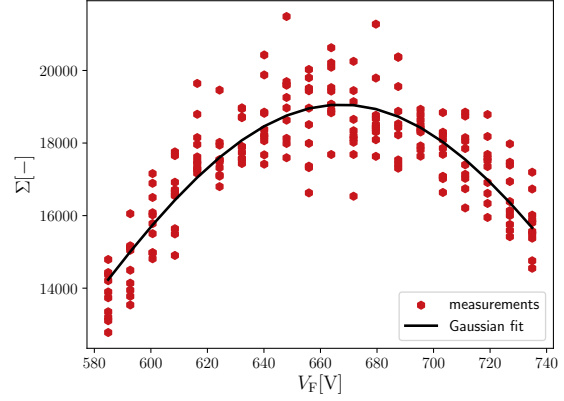
Figure 6. Auto-focus result: \Sigma as a function of focus potential V_F for spot (1,2). Using I_{x,y}^{\text{opt}*}(i,j) determined using a fine I_{x,y} -scan around the I_{x,y}^{\text{opt}*}(i,j) -values obtained in the I_{x,y} -scan of step 1 (see figure 5), we sweep the focus potential of the electron source in order to obtain the optimum focus for the windows, V_F^{\text{opt}}(i,j) , equalling V_F for which \Sigma is maximised. The dots correspond to the measured values and the line is a one-dimensional Gaussian fit to the data.
