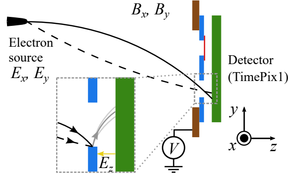
Figure 9. In order to interpret the satellites and the banana-shaped feature, we use the electrostatic deflectors of the electron source ( E ). The continuous and dashed lines indicate the trajectories of the electron beam for two different ( B , E )-settings, each passing through the open window. As such it can be understood that the location where PEs hit the TimePix1-detector are influenced by the trajectory's ( B , E )-setting. The inset shows the corresponding trajectories of the PEs hitting the sample wall, which we interpret to be responsible for the banana-shaped feature. The emitted SEs are accelerated towards the detector by the E_z -field resulting from the voltage applied onto the sample holder. Since the energy of these SEs is small and the sample is close ( \sim 1 mm) to the detector, they are hardly influenced by the B -field. Hence, it is understood that the location where SEs hit the detector is not influenced by the ( B , E )-settings.
