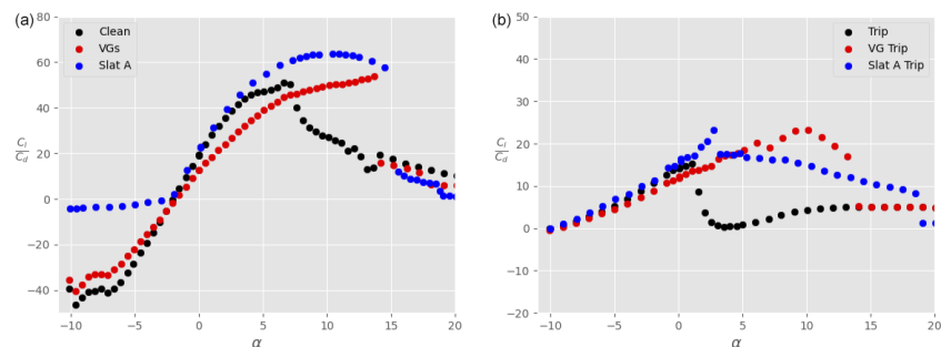
Figure 19. Lift-to-drag ratio C_l/C_d as a function of the angle of attack \alpha for the main airfoil at Re = 1.5 \times 10^6 , without VGs and without slat (black), with VGs only (red), and with slat only in configuration A (blue). (a) Clean airfoil; (b) tripped airfoil.
