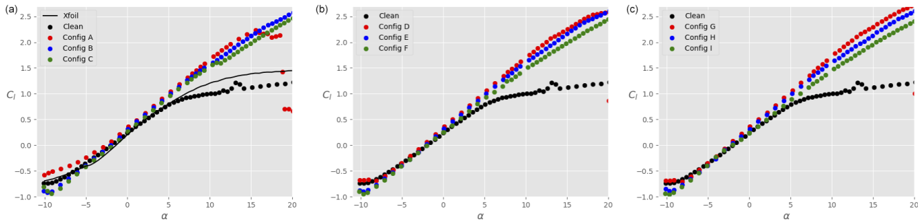
Figure 5. Total lift coefficient C_l on the ensemble airfoil + slat as a function of the angle of attack \alpha for different slat configurations, a clean main airfoil (i.e. no tripping), and Re = 1.5 \times 10^6 : h_{slat}/c_{main} = 0.02 (a), h_{slat}/c_{main} = 0.03 (b), and h_{slat}/c_{main} = 0.04 (c). The black data are taken without slat, while the coloured data are in the presence of a slat with \beta_{slat} = 16.4^\circ (red), \beta_{slat} = 21.4^\circ (blue), and \beta_{slat} = 26.4^\circ (green). The results of Xfoil simulations for the clean main airfoil are shown by the continuous black line (a).
