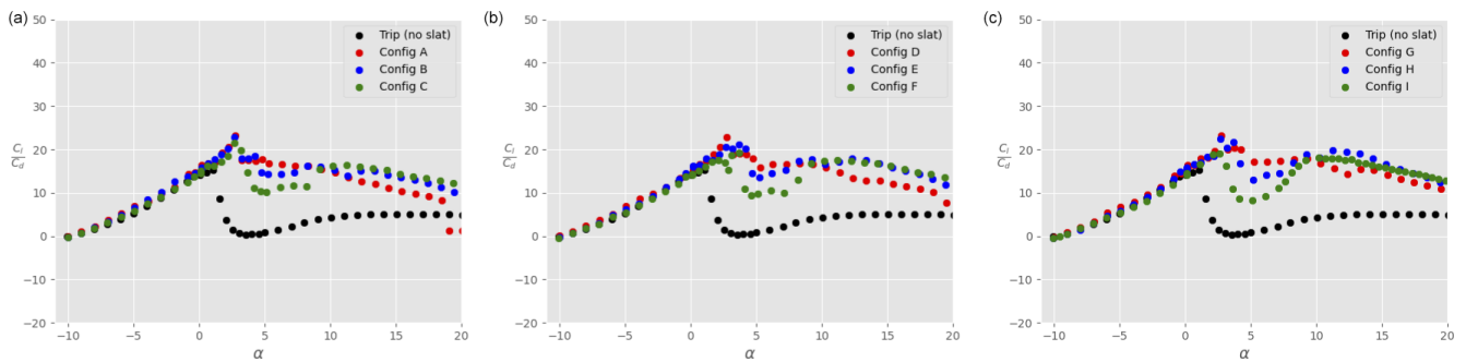
Figure 14. Lift-to-drag ratio C_l/C_d on the ensemble airfoil + slat as a function of the angle of attack \alpha for different slat configurations, a tripped main airfoil, and Re = 1.5 \times 10^6 : h_{\text{slat}}/c_{\text{main}} = 0.02 (a), h_{\text{slat}}/c_{\text{main}} = 0.03 (b), and h_{\text{slat}}/c_{\text{main}} = 0.04 (c). The black data are taken without slat, while the coloured data are in the presence of a slat with \beta_{\text{slat}} = 16.4^\circ (red), \beta_{\text{slat}} = 21.4^\circ (blue), and \beta_{\text{slat}} = 26.4^\circ (green).
