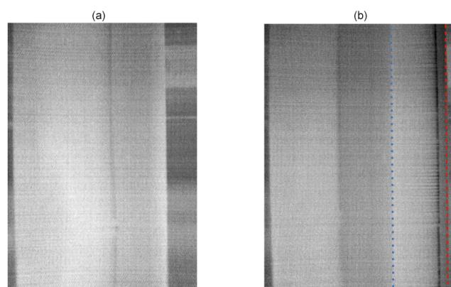
Figure 10. Infrared images of the suction side of the clean main airfoil (i.e. no tripping) at an angle of attack \alpha = 10^\circ : without slat (a) and with slat under configuration A (b). In panel (b), the red dashed line indicates the slat leading edge, whilst the blue dotted line shows the slat trailing edge. Flow is going from right to left.
