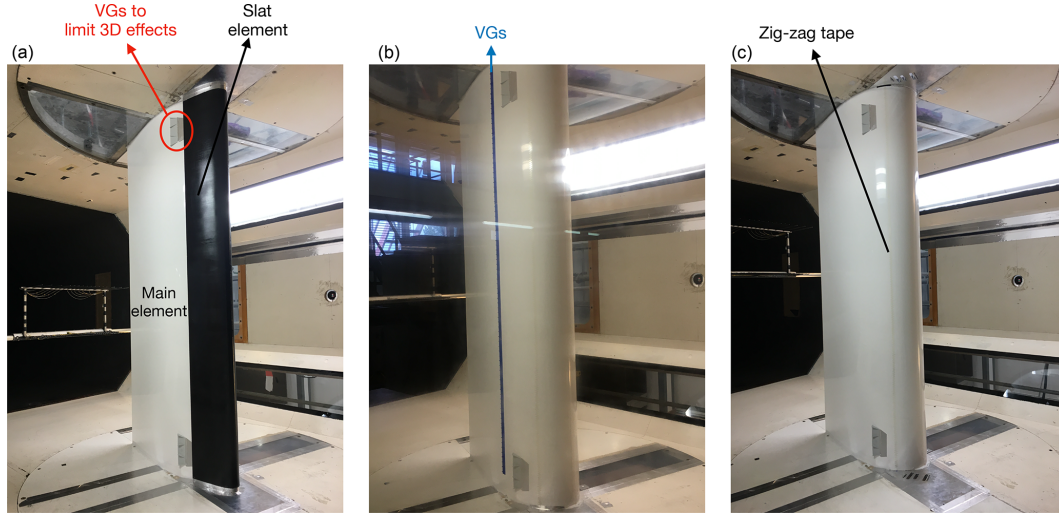
Figure 3. Photographs of the experimental setup: main profile with slat element (a), main profile with vortex generators (b), and main profile with zig-zag tape (c). In all the cases, VGs are used close to the walls to limit three-dimensional effects. This is highlighted in red on the left picture.
