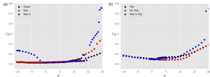
Figure 18. Drag coefficient C_d as a function of the angle of attack \alpha for the main airfoil at Re = 1.5 \times 10^6 , without VGs and without slat (black), with VGs only (red), and with slat only in configuration A (blue). (a) Clean airfoil; (b) tripped airfoil.
