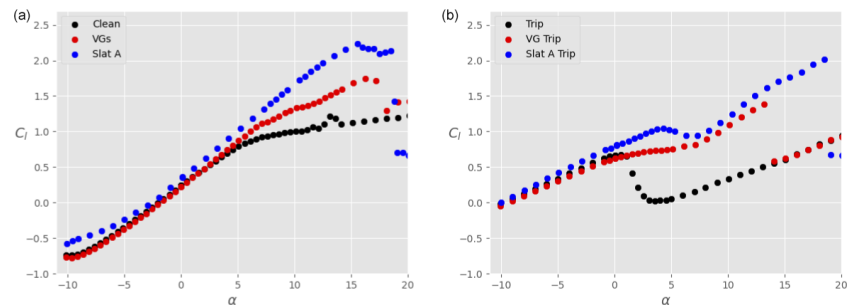
Figure 17. Lift coefficient C_l as a function of the angle of attack \alpha for the main airfoil at Re = 1.5 \times 10^6 , without VGs and without slat (black), with VGs only (red), and with slat only in configuration A (blue). (a) Clean airfoil; (b) tripped airfoil.
