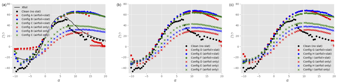
Figure 8. Lift-to-drag ratio C_l/C_d as a function of the angle of attack \alpha for different slat configurations, a clean main airfoil (i.e. no tripping), and Re = 1.5 \times 10^6 : h_{\text{slat}}/c_{\text{main}} = 0.02 (a), h_{\text{slat}}/c_{\text{main}} = 0.03 (b), and h_{\text{slat}}/c_{\text{main}} = 0.04 (c). The black data are taken without slat, while the coloured data are in the presence of a slat with \beta_{\text{slat}} = 16.4^\circ (red), \beta_{\text{slat}} = 21.4^\circ (blue), and \beta_{\text{slat}} = 26.4^\circ (green). Furthermore, dots represent the total lift coefficient (main airfoil + slat), whilst the crosses show the lift force on the main airfoil only. The results of Xfoil simulations for the clean main airfoil are shown by the continuous black line in panel (a).
