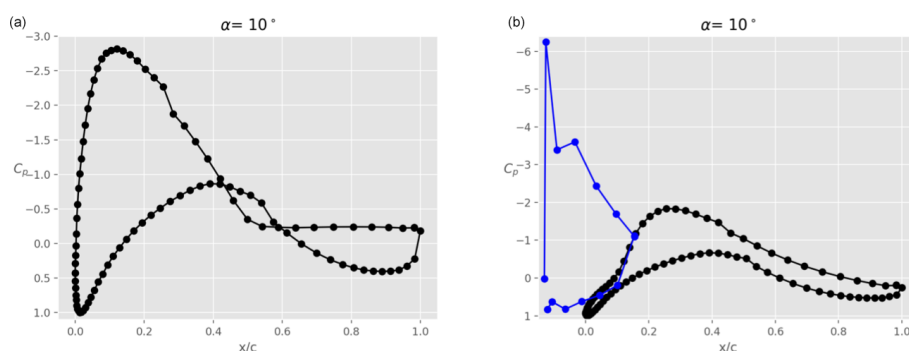
Figure 9. Pressure coefficient C_p at \alpha = 10^\circ for a clean main airfoil (i.e. no tripping): main airfoil alone (a) and main airfoil with slat in case A (b), where both the pressure distributions on the main airfoil (black) and slat (blue) are shown.
