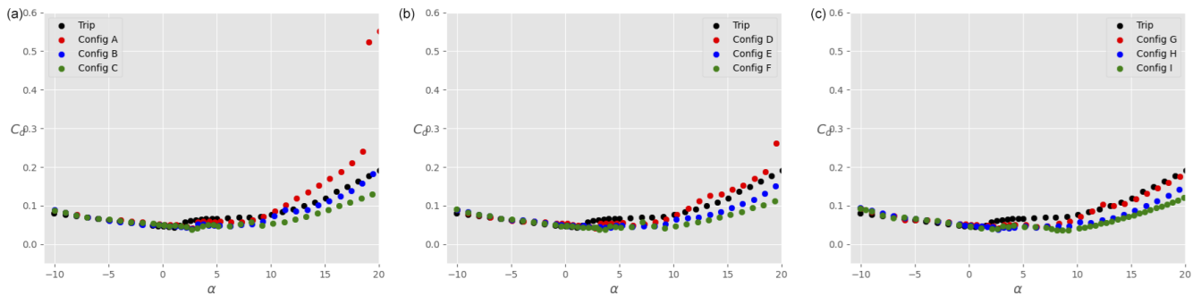
Figure 13. Total drag coefficient C_d on the ensemble airfoil + slat as a function of the angle of attack \alpha for different slat configurations, a tripped main airfoil, and Re = 1.5 \times 10^6 : h_{\text{slat}}/c_{\text{main}} = 0.02 (a), h_{\text{slat}}/c_{\text{main}} = 0.03 (b), and h_{\text{slat}}/c_{\text{main}} = 0.04 (c). The black data are taken without slat, while the coloured data are in the presence of a slat with \beta_{\text{slat}} = 16.4^\circ (red), \beta_{\text{slat}} = 21.4^\circ (blue), and \beta_{\text{slat}} = 26.4^\circ (green).
