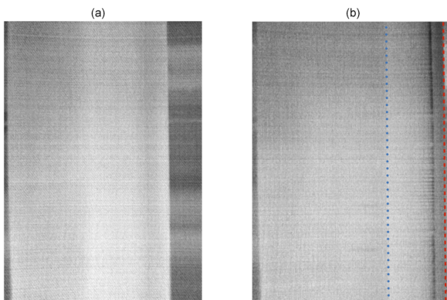
Figure 15. Infrared images of the suction side of the tripped main airfoil at an angle of attack \alpha = 10^\circ : without slat (a) and with slat under configuration A (b). In panel (b), the red dashed line indicates the slat leading edge, whilst the blue dotted line shows the slat trailing edge.
