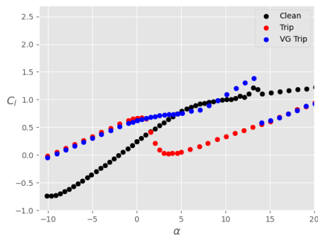
Figure 12. Lift coefficient C_l as a function of the angle of attack \alpha for a main element without slat: clean airfoil without VGs (black), tripped airfoil without VGs (red), and tripped airfoil with VGs (blue).
