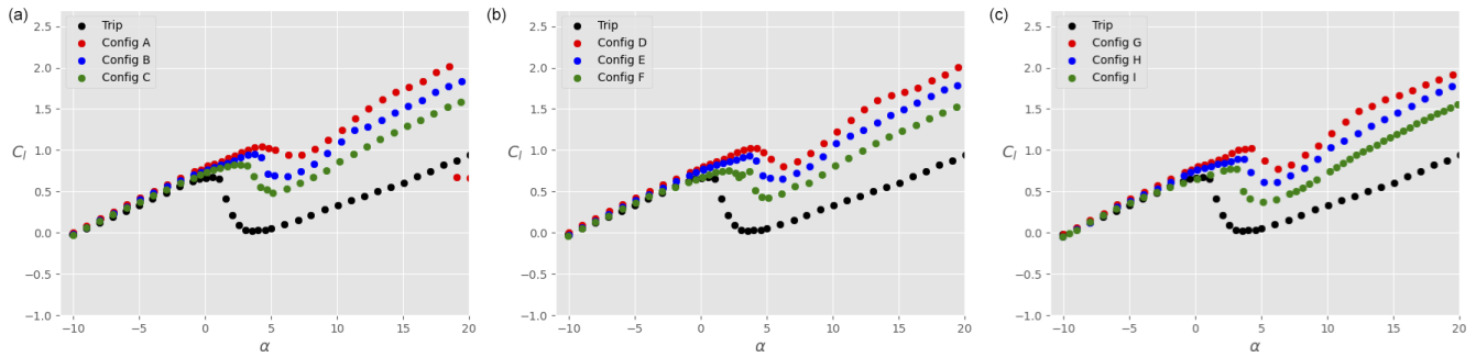
Figure 11. Total lift coefficient C_l on the ensemble airfoil + slat as a function of the angle of attack \alpha for different slat configurations, a tripped main airfoil, and Re = 1.5 \times 10^6 : h_{\text{slat}}/c_{\text{main}} = 0.02 (a), h_{\text{slat}}/c_{\text{main}} = 0.03 (b), and h_{\text{slat}}/c_{\text{main}} = 0.04 (c). The black data are taken without slat, while the coloured data are in the presence of a slat with \beta_{\text{slat}} = 16.4^\circ (red), \beta_{\text{slat}} = 21.4^\circ (blue), and \beta_{\text{slat}} = 26.4^\circ (green).
