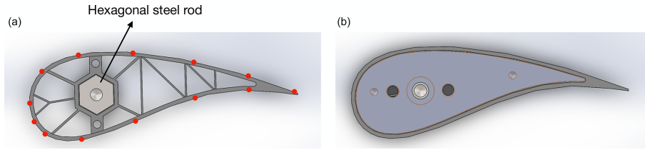
Figure 2. CAD design of the slat cross-section (a) and end plate (b). Red dots on the left figure indicate the location of the pressure tabs.
