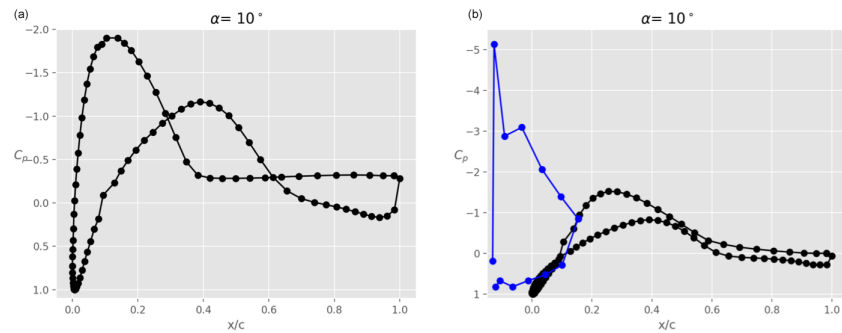
Figure 16. Pressure coefficient C_p at \alpha = 10^\circ for a tripped main airfoil: main airfoil alone (a) and main airfoil with slat in case A (b), where both the pressure distributions on the main airfoil (black) and slat (blue) are shown.
