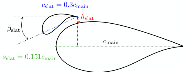
Figure 1. Illustration of the slat parameters of interest in this work: (i) gap width h_{\text{slat}} between the main airfoil and the slat and (ii) the slat angle \beta_{\text{slat}} relative to the main airfoil.
