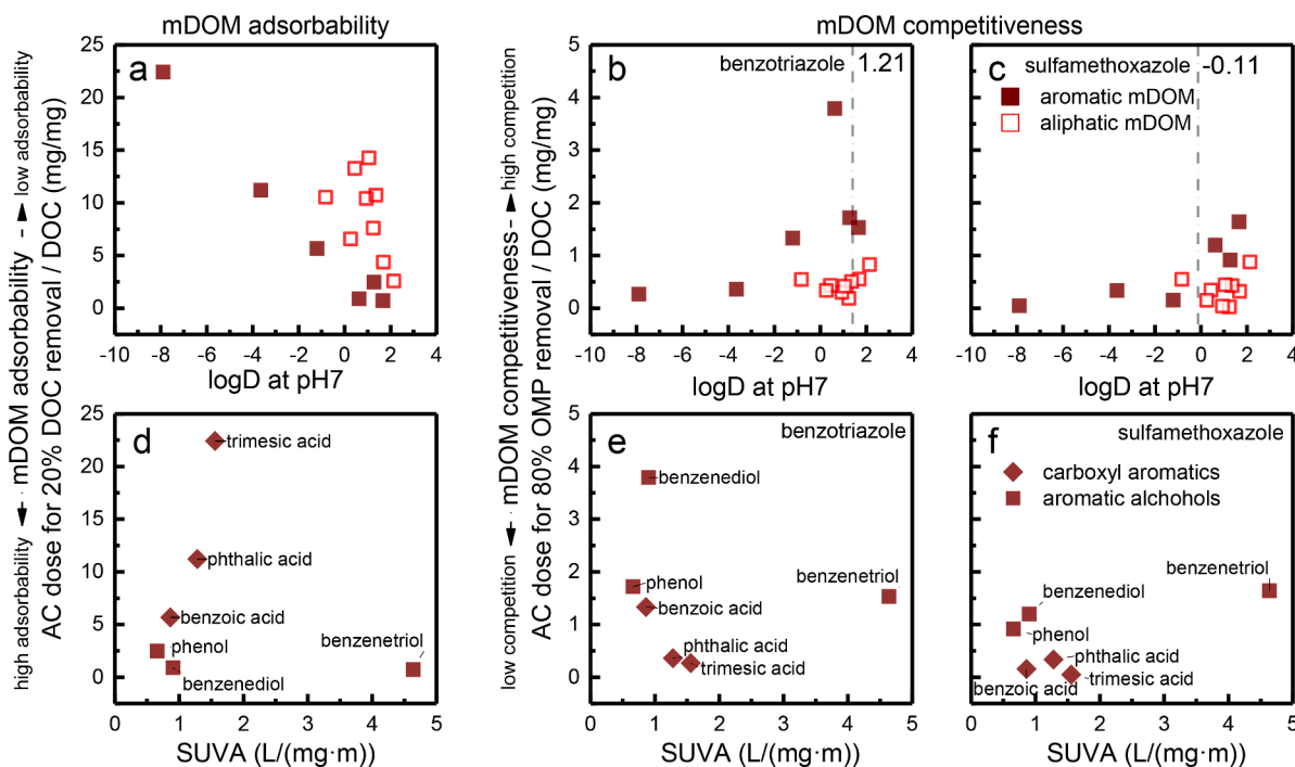
Fig. 3. mDOM adsorbability versus logD (a) and SUVA (d), and mDOM competitiveness versus logD and SUVA for benzotriazole (b,e) and sulfamethoxazole (c,f), respectively. Data for other four OMPs (iopromide, carbamazepine, diclofenac, bezafibrate) in Fig. S4. mDOM competitor names omitted in a–c due to reasons of clearness to the caption. Reference lines in subfigure b/c showing the logD of the specific OMP at pH 7. The adsorption time was 48 h.
