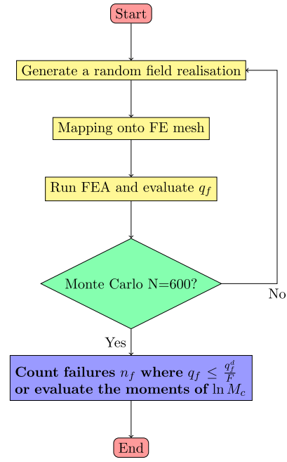
Figure 5. Flowchart for calculating p_f in Equation (2).
