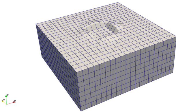
Figure 1. Deformed finite element mesh ( 5 \times 5 \times 2 \text{ m} ) for a square footing (deformation enlarged by a factor of 3 and footing width B = 1.0 \text{ m} ).
