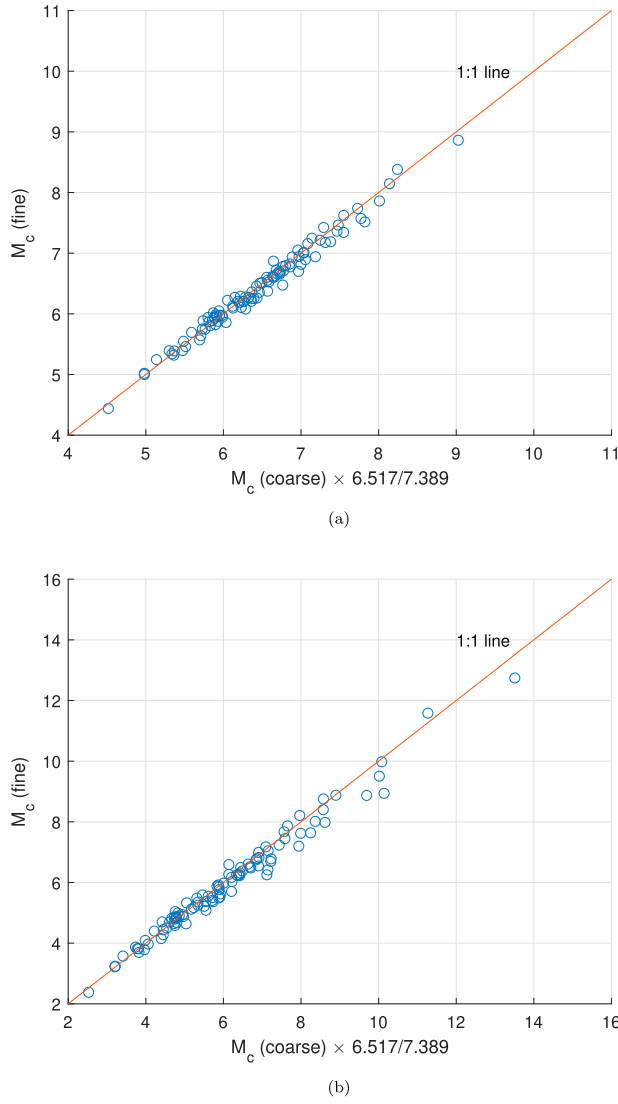
Figure 2. M_c based on the coarse mesh versus M_c based on the fine mesh for \theta_{\text{In } c_u} = 2.0 \text{ m} ( N = 100 ): (a) \text{COV} = 0.2 ; (b) \text{COV} = 0.5 .
