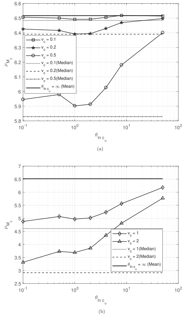
Figure 4. \mu_{M_c} versus \theta_{\text{In } c_u} (lower and upper bounds based on median and mean indicated as lines without markers): (a) \text{COV} = 0.1, 0.2, 0.5 ; (b) \text{COV} = 1.0, 2.0 .
