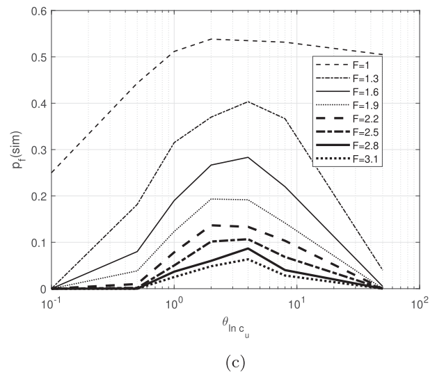
Figure 11. Simulated probabilities versus SOF for different F (relative to q_r^* ) and CPT sampling location, \text{COV} = 1.0 ( B = 1.0 m): (a) r/B = 0 ; (b) r/B = \sqrt{2} \times 0.5 ; (c) r/B = \sqrt{2} \times 1.5 .
