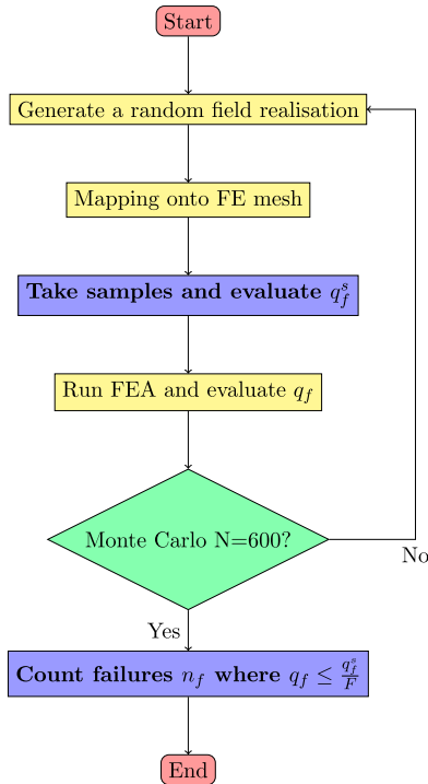
Figure 9. Flowchart for calculating p_f in Equation (4) (the difference to Figure 5 is shown in bold).
