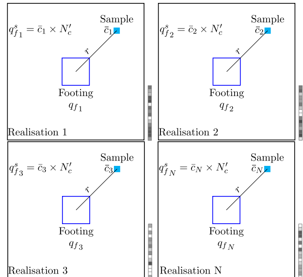
Figure 8. Plan view of the soil domain showing the position of a vertical sample relative to the square footing; the vertical sample consists of n = 16 random cells, as shown to the right of each realisation.
