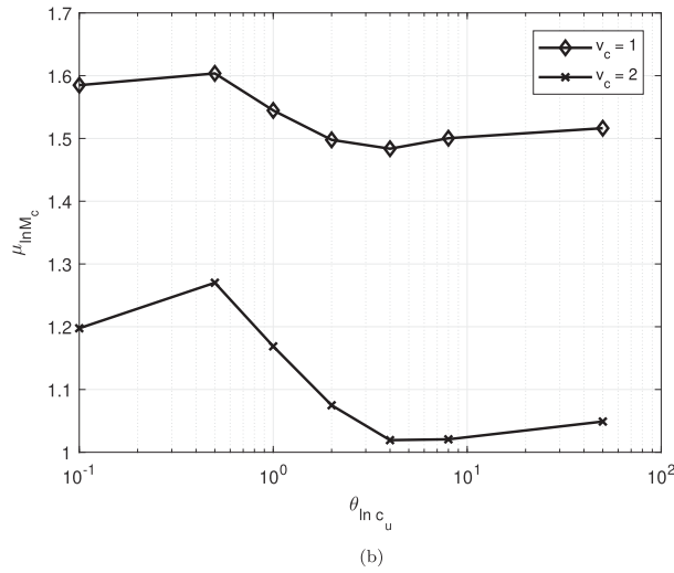
Figure 6. \mu_{\ln M_c} versus \theta_{\ln c_u} : (a) \text{COV} = 0.1, 0.2, 0.5 ; (b) \text{COV} = 1.0, 2.0 .
