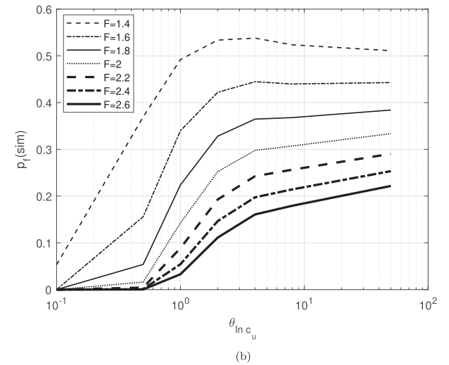
Figure 7. Simulated probabilities versus SOF for different F (relative to deterministic q_f ) and COV: (a) \text{COV} = 0.5 ; (b) \text{COV} = 1.0 .
