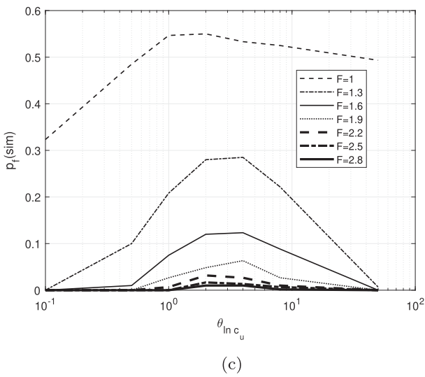
Figure 10. Simulated probabilities versus SOF for different F (relative to q_r^* ) and CPT sampling location, \text{COV} = 0.5 ( B = 1.0 m): (a) r/B = 0 ; (b) r/B = \sqrt{2} \times 0.5 ; (c) r/B = \sqrt{2} \times 1.5 .
