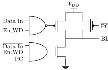
Figure 2.33: The electrical model of an the write driver and precharger used in this thesis.
