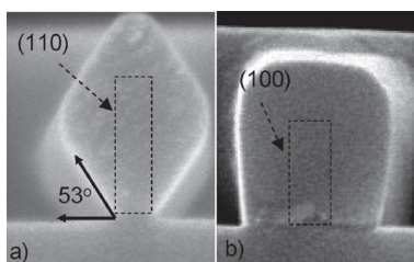
Figure 2.24: Cross sectional SEM images on fins after epitaxial growth on (a) \langle 110 \rangle side wall surface and (b) \langle 100 \rangle sidewall surface [9].
