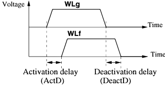
(a) Faulty behaviors in a self-timed WL signal.
