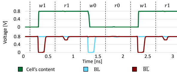
Figure 3.7: Electrical waveforms when simulating a cell affected by OC08 = 25 kΩ.
