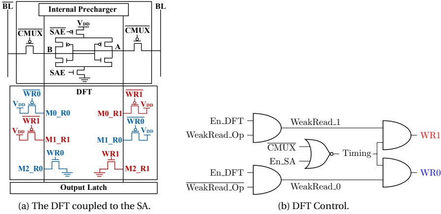
Figure 4.11: DFT Organization.
