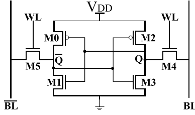
Figure 2.30: The electrical model of an SRAM 6T cell.
