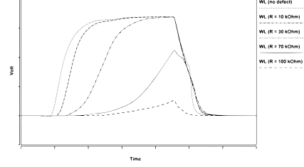
(b) Faulty behaviors in a WL with fixed deactivation time.
