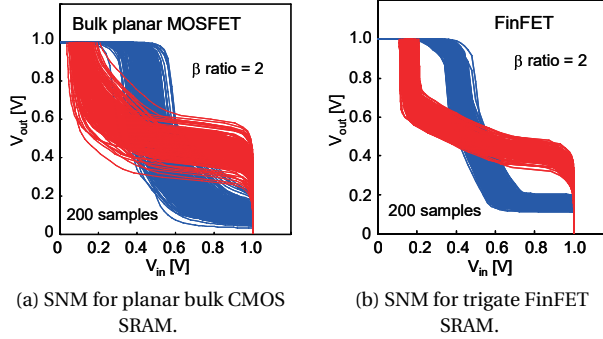
Figure 2.35: SRAM butterfly curves for bulk planar and FinFET. The FinFET SRAM exhibits superior SNM thanks to smaller V_{th} variation due to its undoped channel [88].
