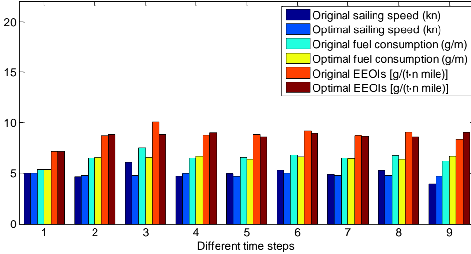
Fig. 13 The navigation optimization results of the 5# ship
