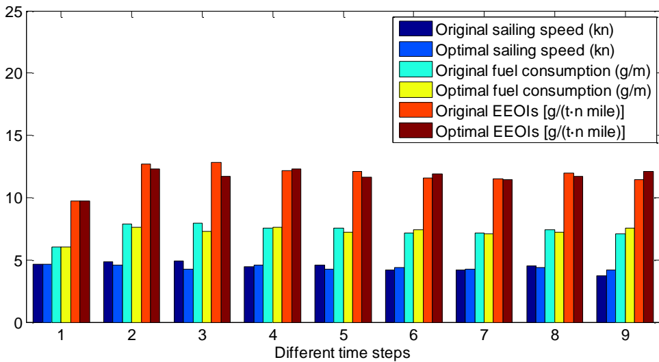
Fig. 11 The navigation optimization results of the 3# ship
