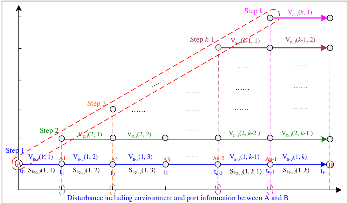
Fig. 3 The dynamic optimization process for fleet energy consumption
