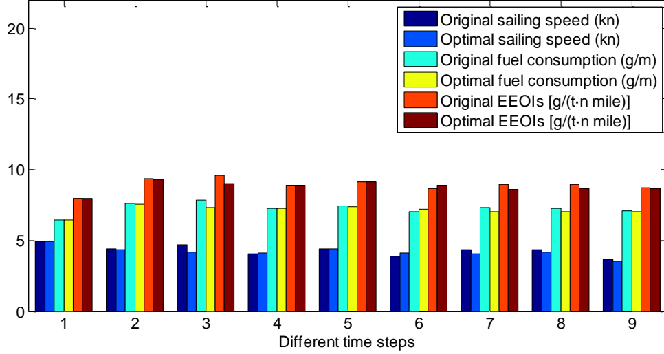
Fig. 12 The navigation optimization results of the 4# ship
