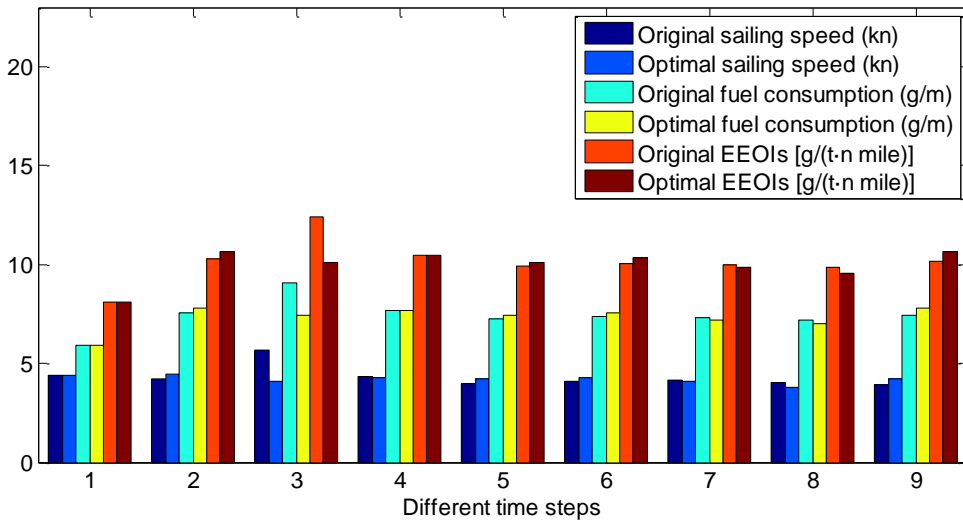
Fig. 10 The navigation optimization results of the 2# ship
