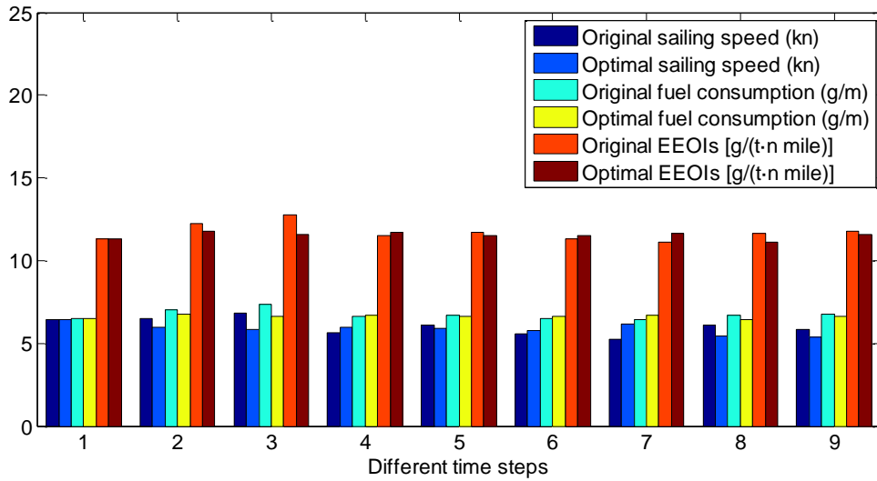
Fig. 9 The navigation optimization results of the 1# ship
