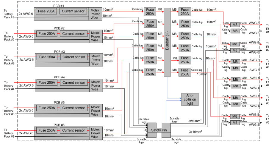
Figure 11. The robustified electric architecture of the DEP-SFD2.
