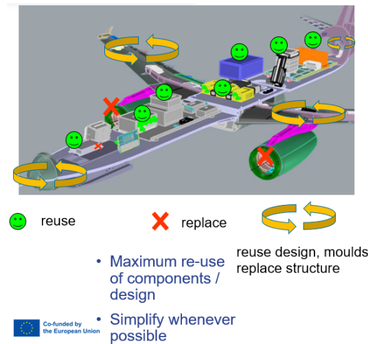
Figure 3. The design philosophy for the D08 DEP-SFD.
