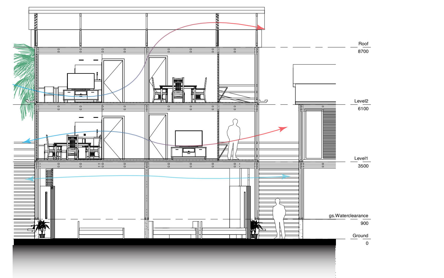
Section 1:100
