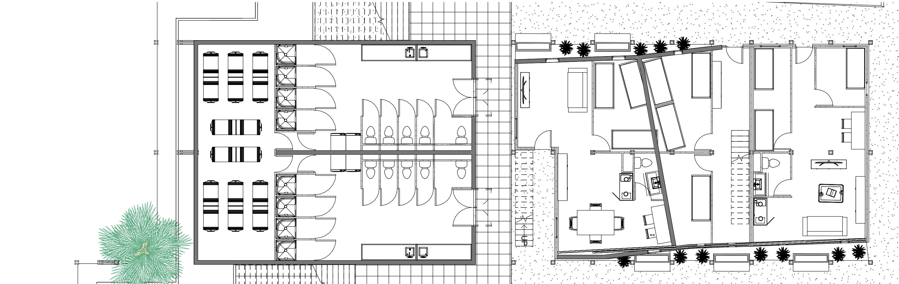
Floorplan groundfloor 1:100
