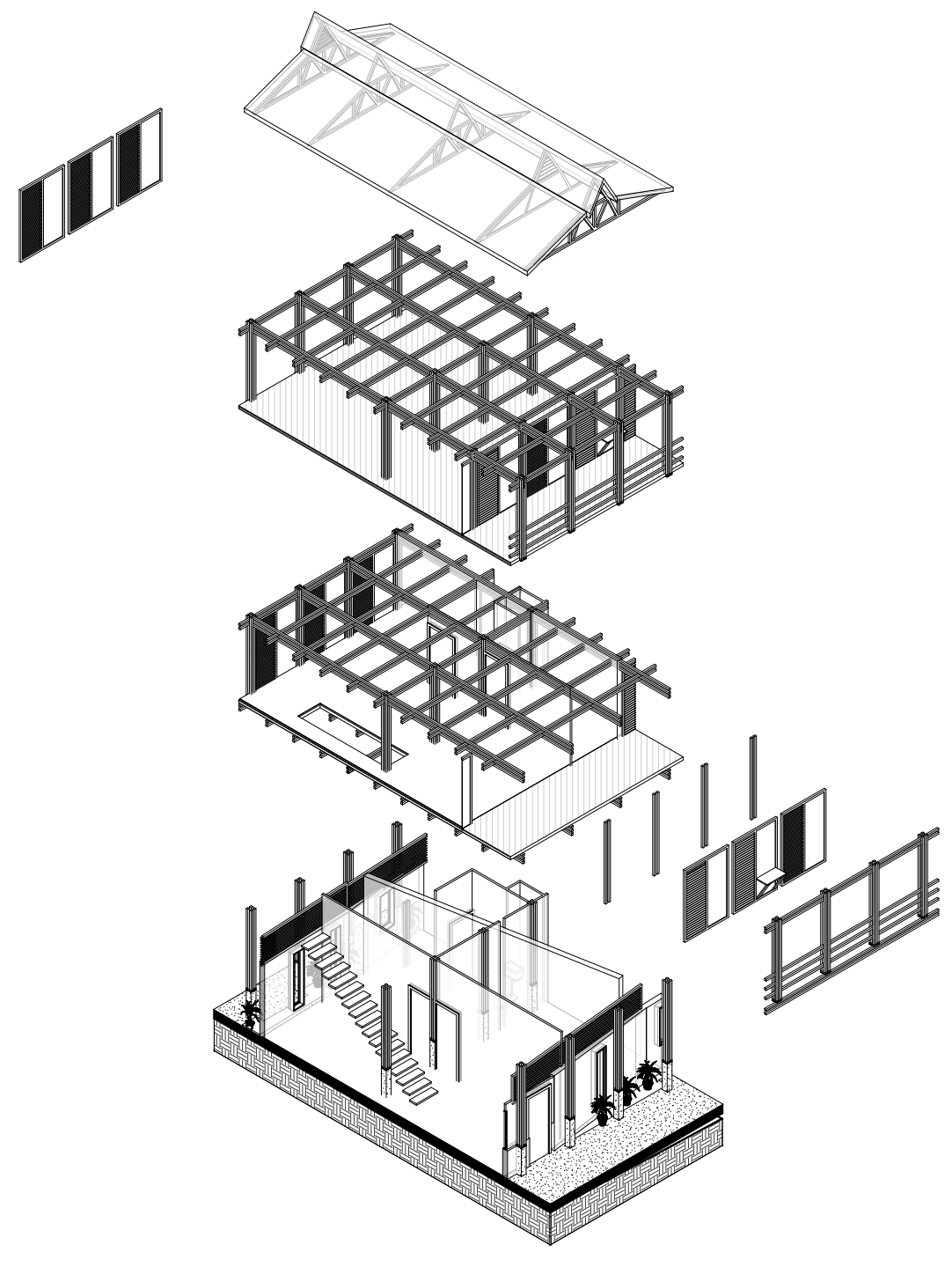
Exploded view
