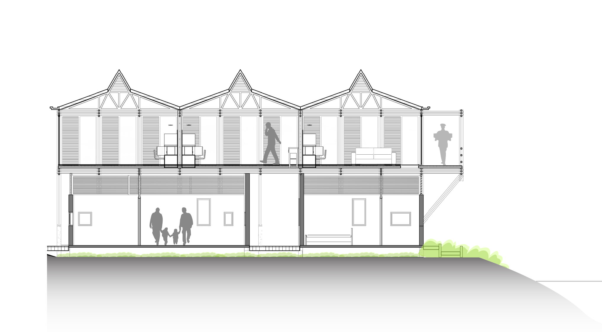
Section 1:100
