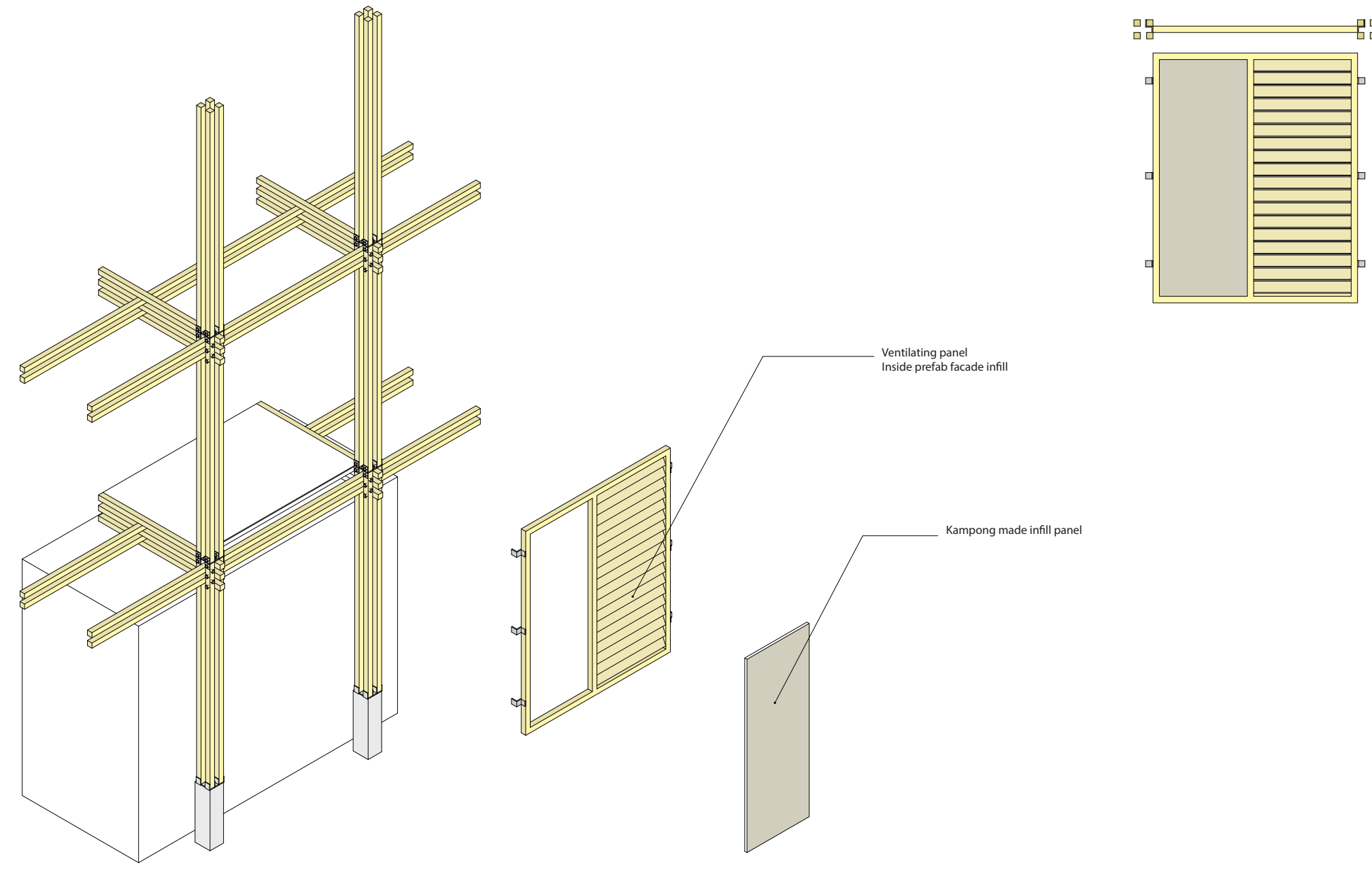
Exploded view structure with infill
