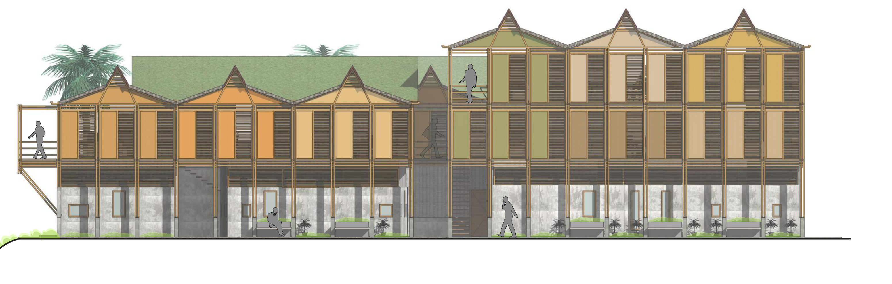
Facade 1:100
