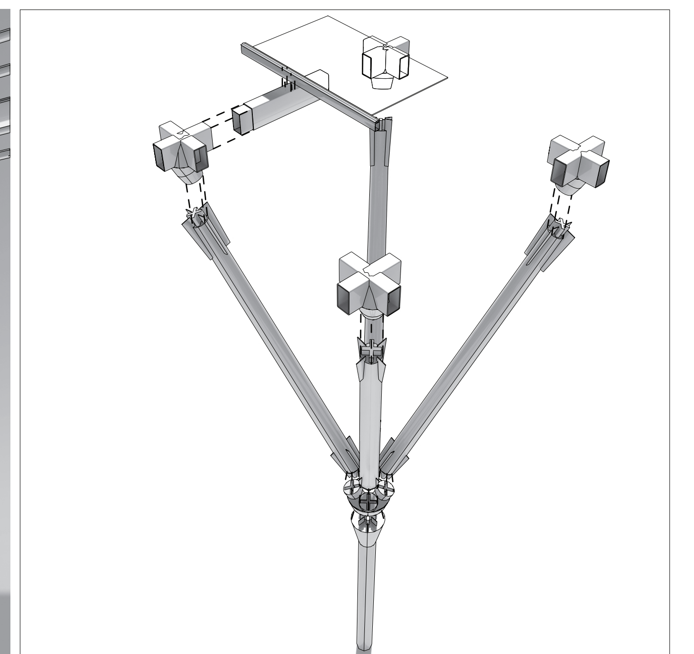
Axonometrie stationshalkolom
