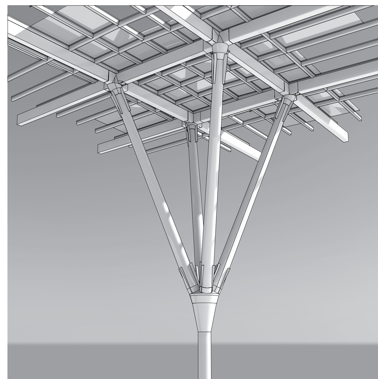
Isolering middenkolom stationshal
