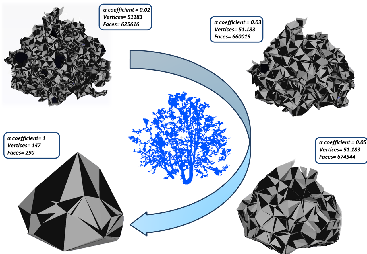
Fig 6. Canopy envelop results using different \alpha coefficients from the triangulation mesh (the best result is obtained by \alpha = 0.05 ).
