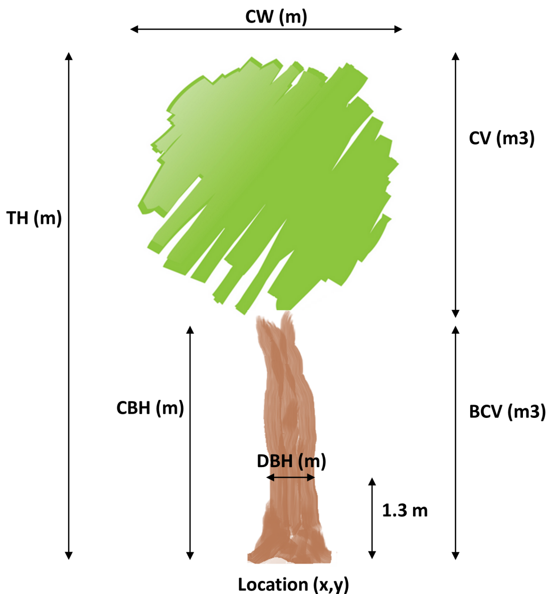
Fig 1. Schema of tree parameters. Location coordinates (x, y), Tree Height (TH), Crown Width (CW), Diameter at Breast Height (DBH), Crown Base Height (CBH), Base Crown Volume (BCV) and Canopy Volume (CV).
