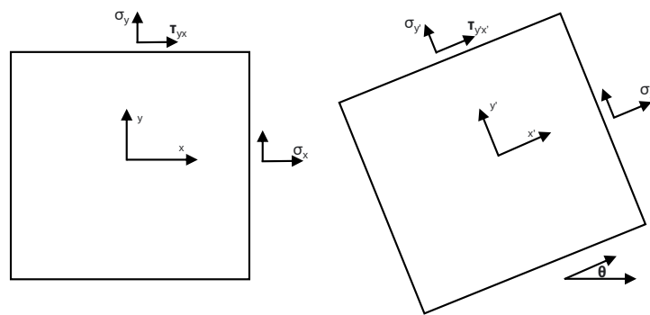
Figure 3. Stress transformation for a plane inclined at an angle.
