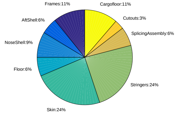
(b) Composite, M_{\text{fuselage}} = 7790\text{kg}
