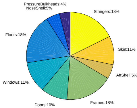
(a) Aluminum fuselage, M_{\text{fuselage}} = 9655\text{kg}
