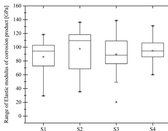
Fig. 18. Range of E_{cp} per specimen, represented by each box. The top, middle and bottom line of the boxes correspond to the 75-, 50- and 25-percentile value ( \times 75 , \times 50 and \times 25 ) respectively. The whiskers show the minimum and maximum values, while crosses represent outliers.
