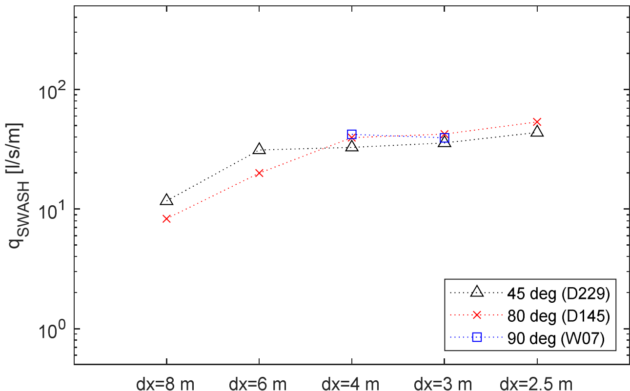
Figure 5. The mean overtopping discharges with different grid sizes ( dx = 2.5 to 8 m) for different wave directions (45, 80 and 90 degrees) to check the grid conversion. Directions of 45 and 80 degrees are the cases with long-crested waves, while directions of 90 degrees correspond to the cases with short-crested waves.
