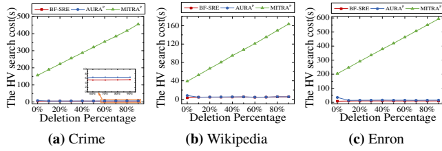
Figure 6: Comparison of search time costs of BF-SRE, AURA P , and MITRA P on the highest-volume (HV) keyword with deletion percentage (namely, delete 0-90% pairs).
