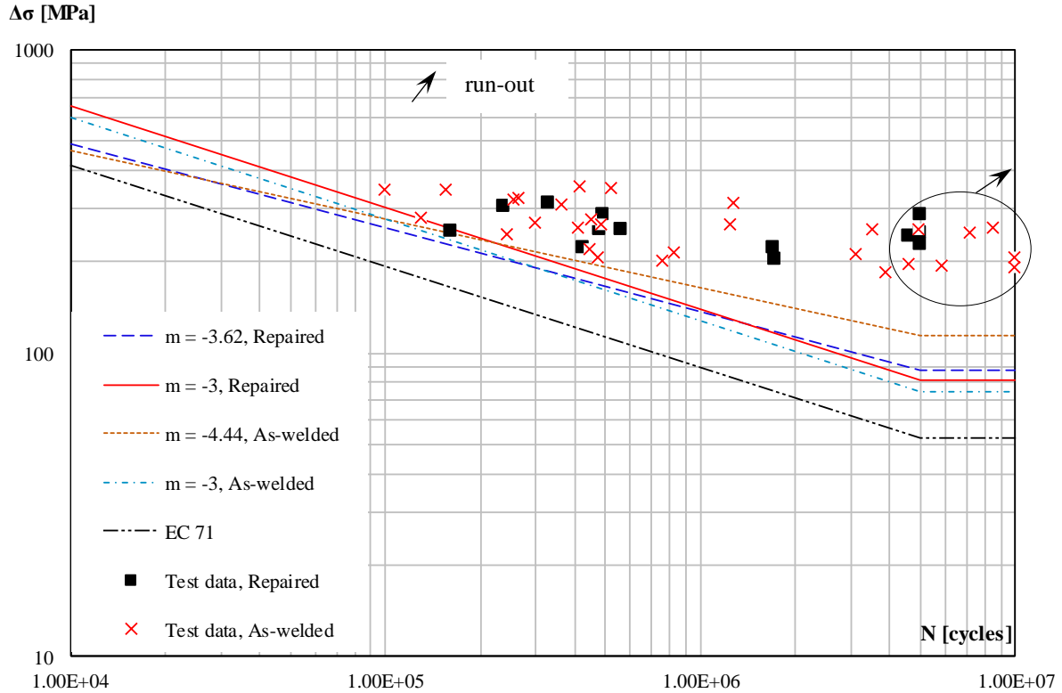
Figure 10. Comparison between S-N curves of weld toe crack in rolled steels of repaired and in the as-welded specimens.
