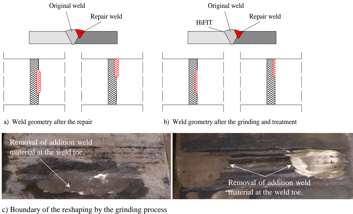
Figure 8. Weld shape after the repair and the repaired weld geometry after reshaping and HiFIT.
