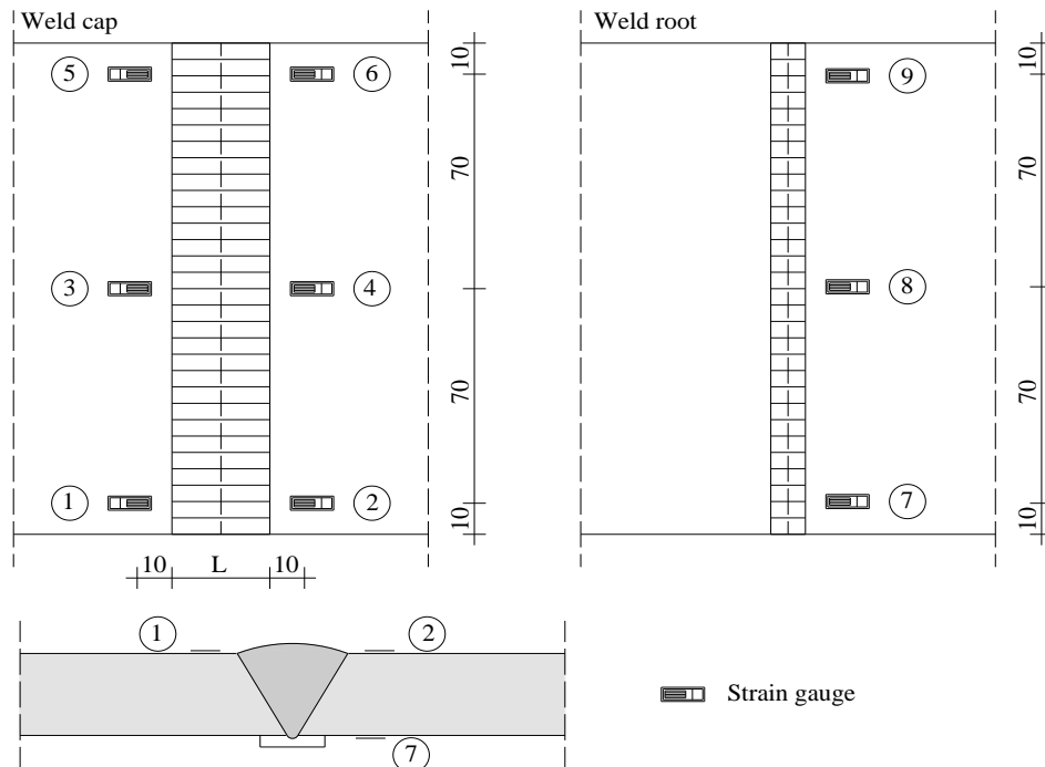
Figure 3. Strain gauge configuration on a test specimen.
