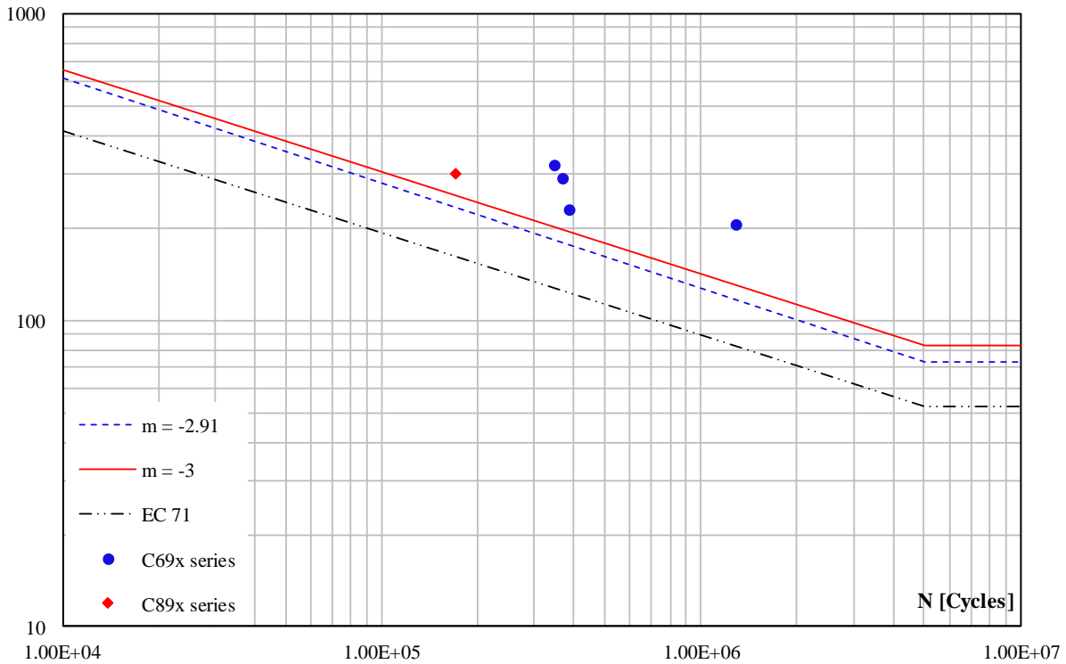
Figure 11. S-N curves of weld toe cracks in cast steels of the repaired V-shape welded specimens.
