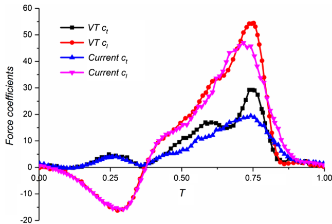
Fig. 5 Force coefficient comparison between the numerical solver of Viswanath et al. and the current IBM solver.
