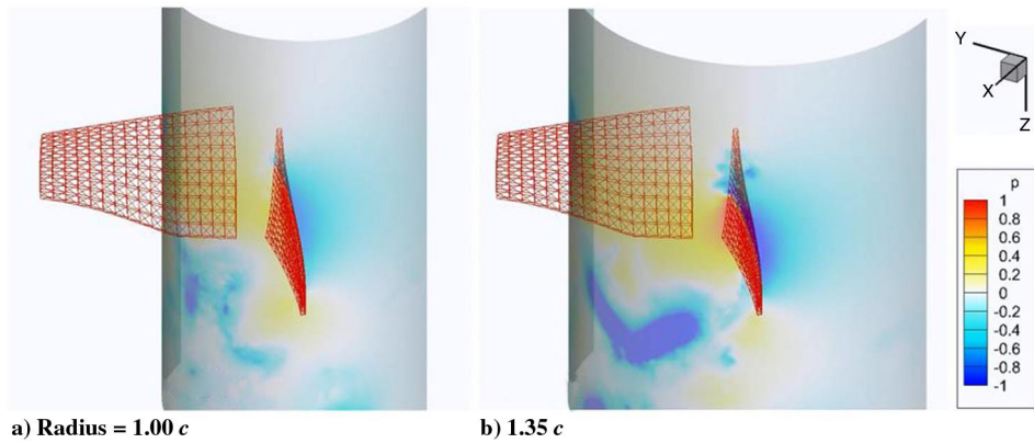
Fig. 17 Pressure contours at radii of a) 1.00c and b) 1.35c .
