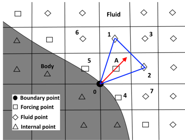
Fig. 3 Possible interpolation template for the forcing point.
