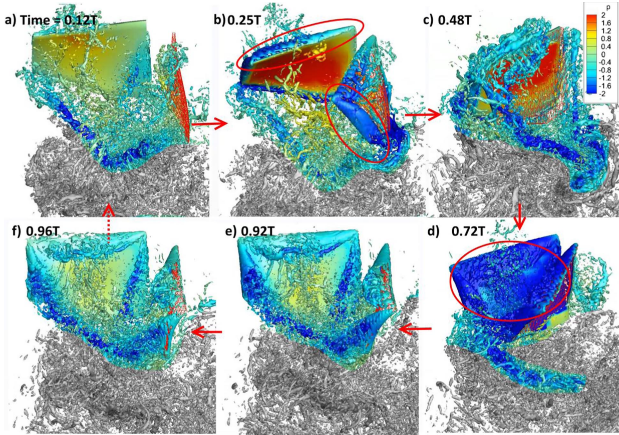
Fig. 15 Isosurface plotted at Q criterion of 100 superimposed with pressure contour from numerical simulation over one period.
