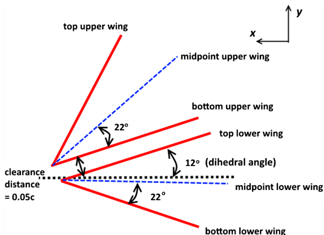
Fig. 9 Geometric flapping parameters of the DelFly's wings from the frontal view.
