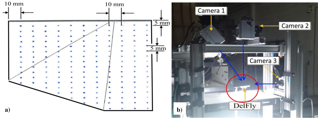
Fig. 2 Representations of a) DelFly wing with dots; and b) experimental setup for the wing deformation capture, adapted from the work of Deng et al. [13].
