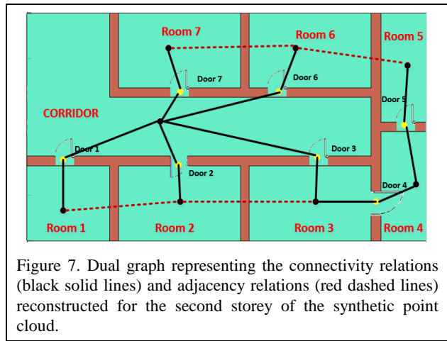
Figure 7. Dual graph representing the connectivity relations (black solid lines) and adjacency relations (red dashed lines) reconstructed for the second storey of the synthetic point cloud.
