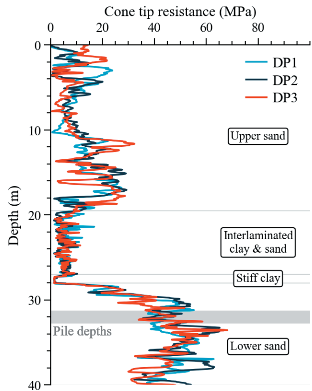
Figure 2: CPTs performed at each driven precast pile prior to installation
