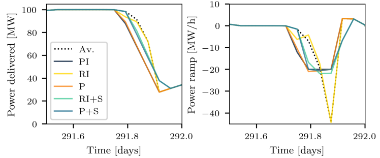
Figure 5. Power delivered and ramp rate for the dispatch calculated with PI, RI, and pessimistic (P) forecasts, and with or without a storage system. The available power (Av.) is marked in black dotted line.
