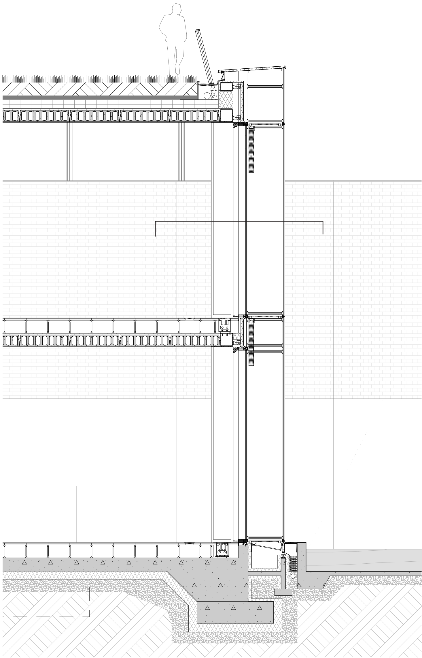
Section
