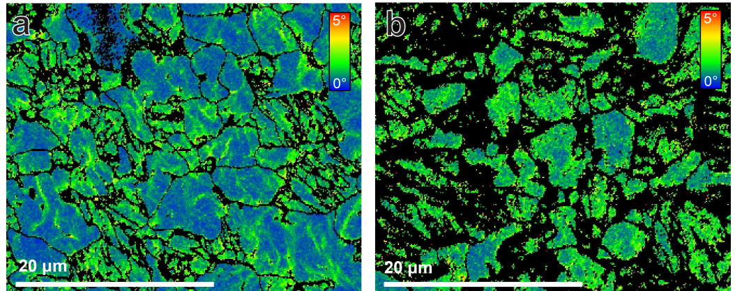
Figure 8. Kernel Average Misorientation (KAM) maps made 150 \mu\text{m} beneath the fracture surface of specimens annealed at (a) 630 ^{\circ}\text{C} and (b) 670 ^{\circ}\text{C} . Black areas signify non-indexed areas, which correspond to either grain boundaries or martensitic regions within the microstructure.
