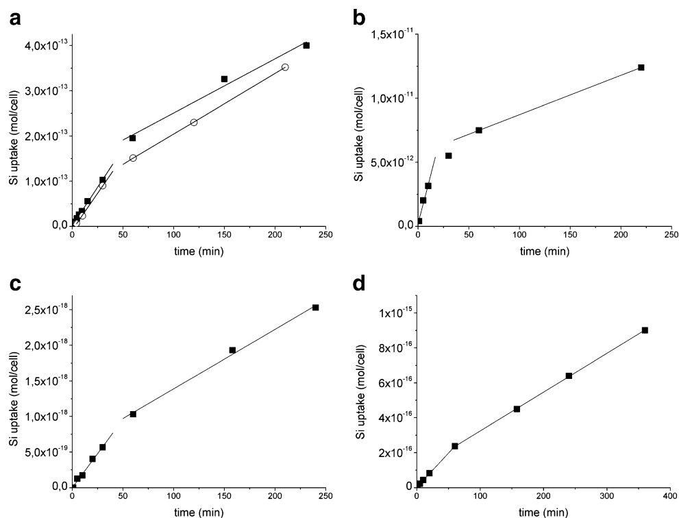
Fig. 1 Silicic acid uptake (in \text{mol cell}^{-1} ) under standard culture conditions by diatom cells following silicic acid addition to Si-limited cells for a Pleurosira laevis (■ 456 or ○ 21 \mu\text{mol/L Si} ), b Coscinodiscus wailesii (456 \mu\text{mol/L Si} ), c Navicula pelliculosa (140 \mu\text{mol/L Si} ), and d N. salinarum (317 \mu\text{mol/L Si} ). Two distinct uptake regimes can be recognized (lines)
