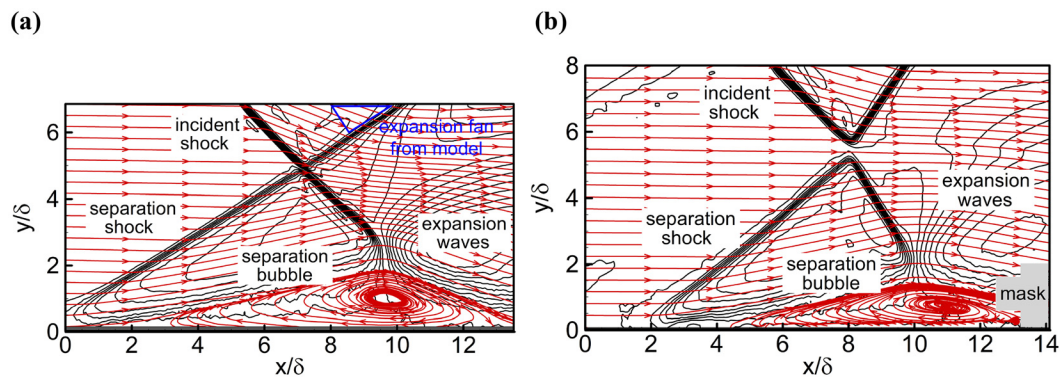
FIG. 8. Time-averaged flow topologies of SWBLIs. (a) Mach 2.5, 21°. (b) Mach 2.0, 17°.
