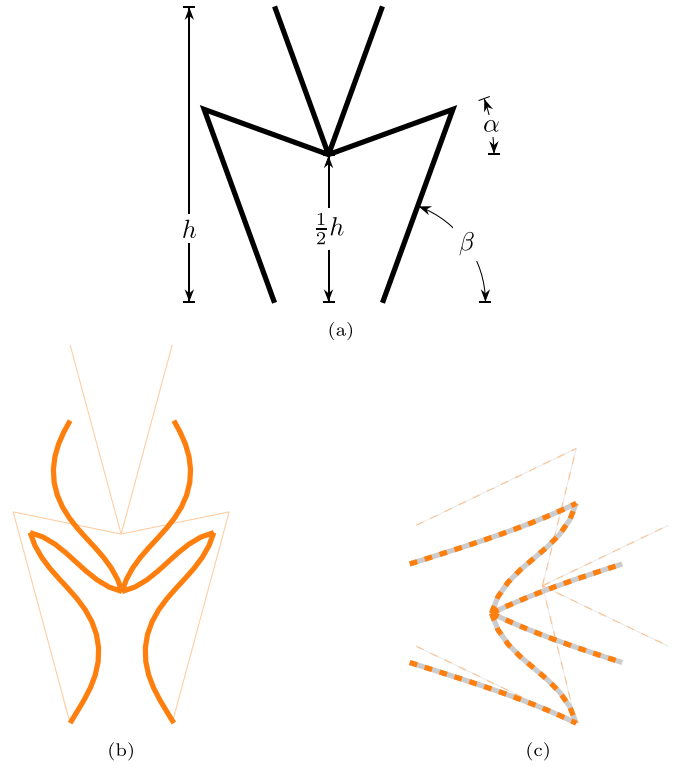
Fig. 2.4. Arrowhead architecture. (a) shows the design and geometric parameters, uniaxial compression is illustrated in (b) for 0° orientation and in (c) for 90° orientation.
