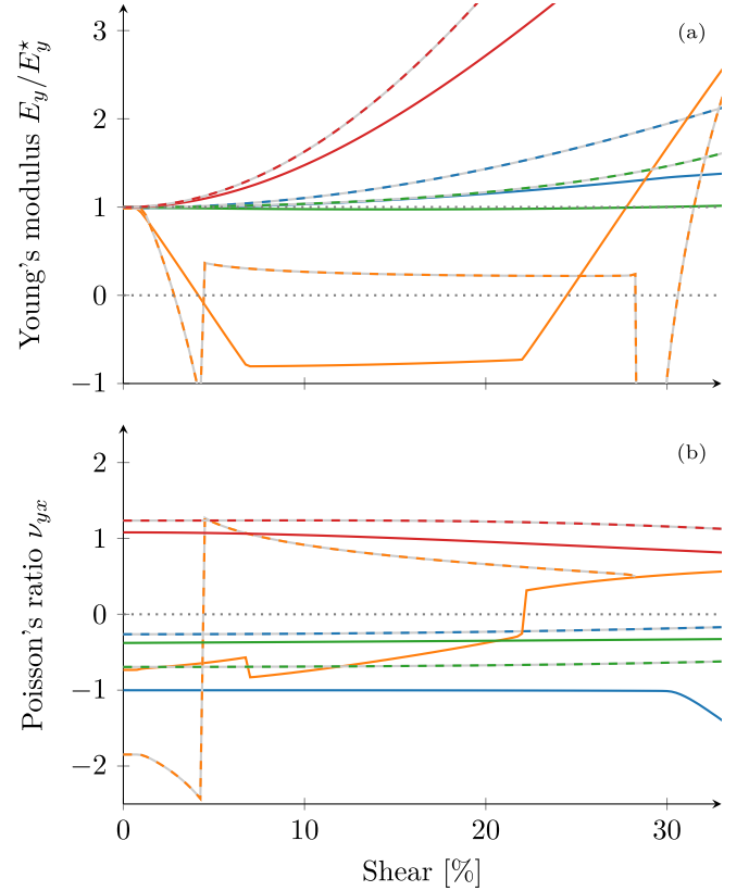
Fig. 4.7. Change of vertical properties under pure shear deformation for different architectures, namely (a) the normalized Young's modulus E_y and (b) the Poisson's ratio \nu_{yx} .
