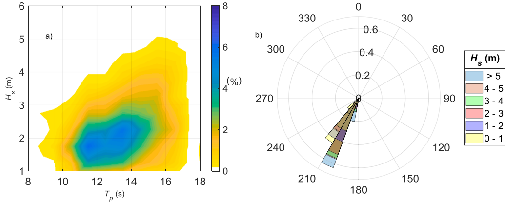
Fig. 8. Wave climate at Torbay, Albany site in Western Australia. The joint occurrence distributions of H_s and (a) T_p ; (b) \beta_m (°).
