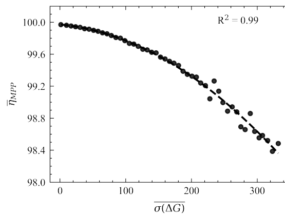
Figure 3. Drop of the binned average efficiency, \bar{\eta}_{MPP} , of the P&O algorithm as a function of the mean irradiance variability in each bin, \overline{\sigma(\Delta G)} . The coefficient of determination ( R^2 ) is included in the graph to indicate the goodness of fit. Other variability metrics can also be fitted with the model. The fitting parameters are given in Appendix A.
