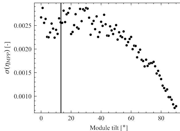
Figure 5. Impact of the module tilt on the daily efficiency for one randomly selected day. For the studied location, the optimal tilt angle is 13.23^\circ , marked with the vertical line.
