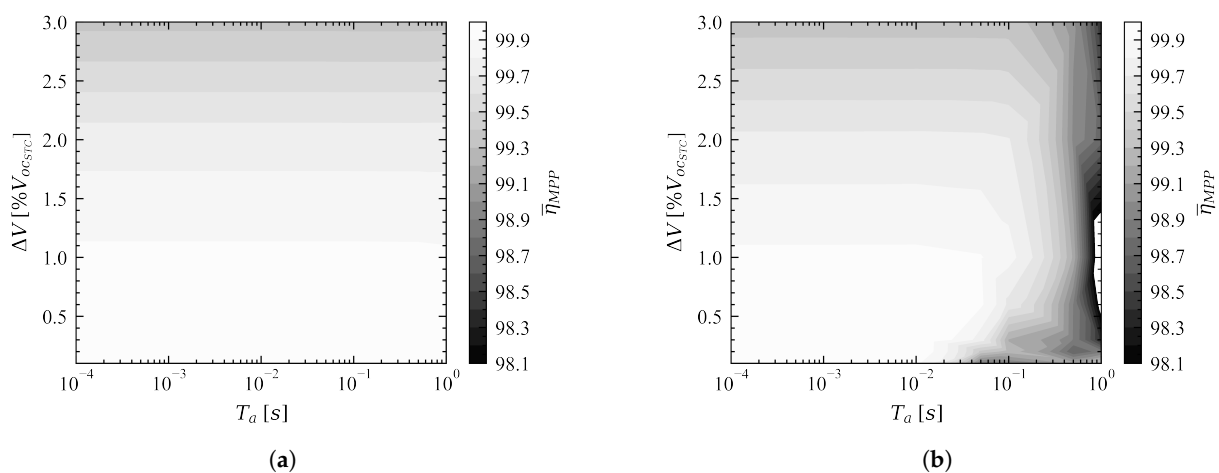
Figure 4. Sensitivity of the P&O algorithm efficiency, \bar{\eta}_{MPP} , to its parameters under (a) clear skies, and (b) variable irradiance.
