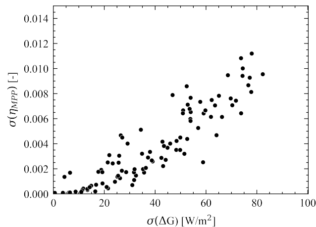
Figure 2. Daily dispersion of differences in irradiance, \sigma(\Delta G) , causes increased daily dispersion of the calculated efficiency, \sigma(\eta_{MPP}) , for 100 randomly selected days. Two outliers were removed for clarity.
