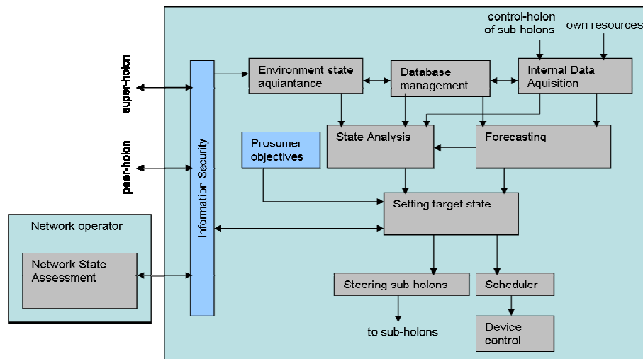
Figure 3. Architecture of a control holon.
