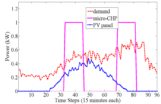
Figure 5. A sample prosumer household demand and production profiles.
