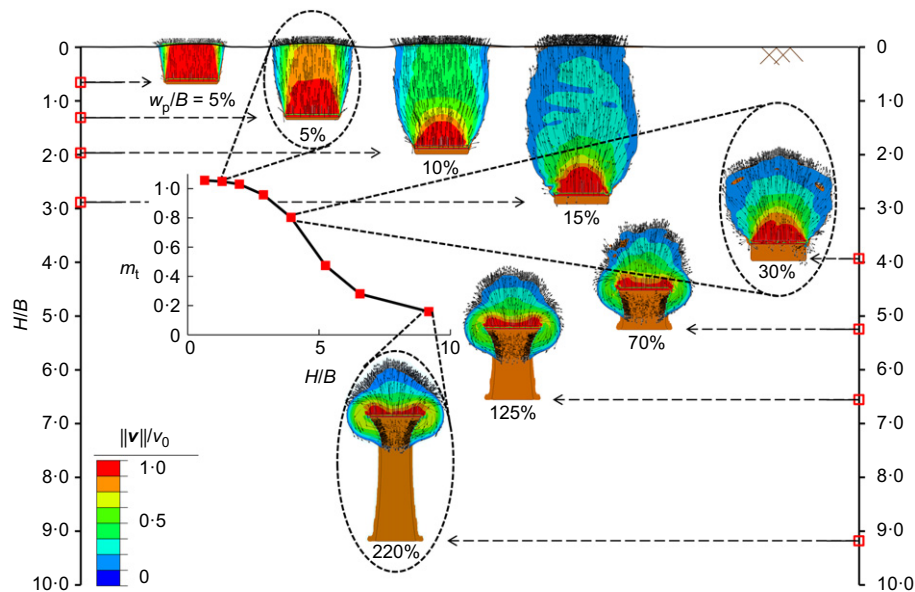
Fig. 8. Variation in the local slope, m_t with embedment depth obtained from the set 1 analysis. The flow velocity ( \|\mathbf{v}\| ) is normalised with respect to the pull-out rate of the anchor ( v_0 )
