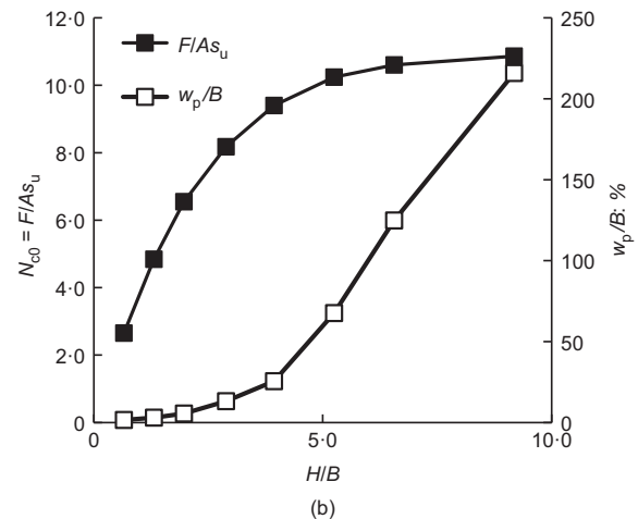
Fig. 3. (a) Variation in continuous pull-out force with increasing displacement of the plate (square symbol represents displacement, w_p , to peak capacity); (b) variation of peak pull-out force and associated displacement for anchor with different embedment ratios in weightless soil ( \gamma'H/s_u = 0 )
