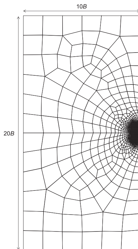
Fig. 1. Schematic diagram of finite-element model (top view)
