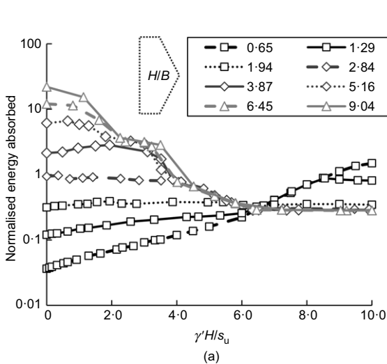
Fig. 7. (a) The normalised energy absorbed by the anchor during pull-out; (b) change in the pull-out displacement as a result of variation in overburden ratio
