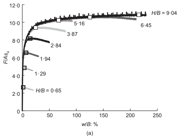
Fig. 3. (a) Variation in continuous pull-out force with increasing displacement of the plate (square symbol represents displacement, w_p , to peak capacity); (b) variation of peak pull-out force and associated displacement for anchor with different embedment ratios in weightless soil ( \gamma'H/s_u = 0 )
