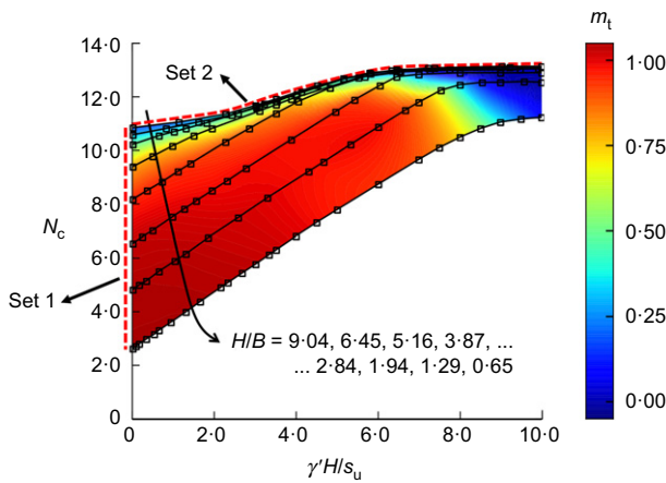
Fig. 11. Variation in the local slope ( m_t ), as a descriptor of anchor failure mode, with anchor embedment depth and overburden ratio
