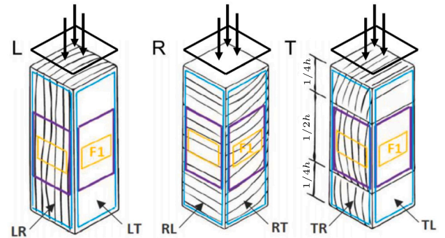
Fig. 3. Exemplary representation of the compression test cubes under compression loading with regard to the alignment in longitudinal, radial or tangential direction [48].
