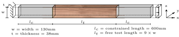
Fig. 12. Tensile test setup with corresponding dimensions according to [7] visualizing the board with fiber deviations.
