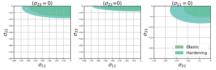
Fig. 2. 2D failure surfaces of the adapted Hill criterion [9], for which the strength and hardening variables are listed in Table 1.
