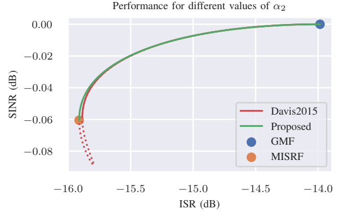
(a) Filter performance in the presence of exclusively white noise and all sidelobes weighted equally.
