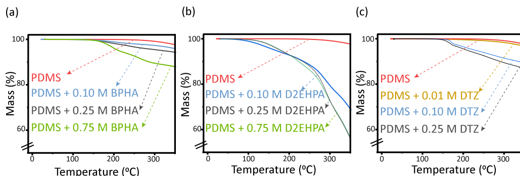
Fig. 4. Quantification of the amount of chelator impregnated in the PDMS beads using thermogravimetry. Thermogravimetry of PDMS beads impregnated with BPHA (a), D2EHPA (b), and DTZ (c) at various concentrations of these chelators in chloroform.
