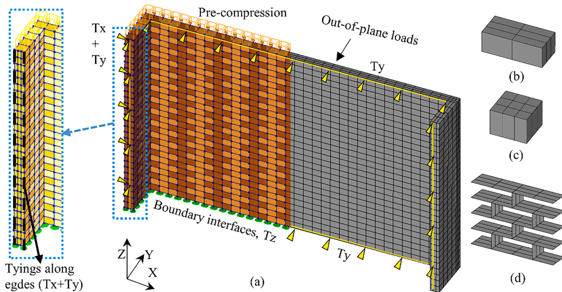
Fig. 5. Modelling settings: (a) geometry, mesh, boundary conditions and loading of the model. Tx, Ty and Tz: d.o.fs constrained in X, Y and Z directions, respectively; (b) mesh of a complete brick; (c) mesh of a half brick at intersection; (d) mesh of interface elements.
