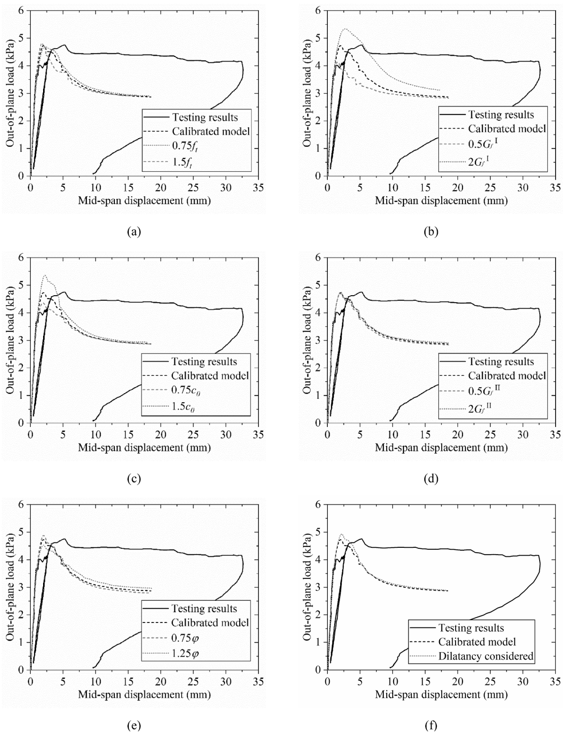
Fig. 9. Material sensitivity study (a)-(f) on: tensile strength f_b , mode-I fracture energy G_f^I , cohesion c_\theta , mode-II fracture energy G_f^{II} , friction angle \varphi and dilatancy angle \psi as single variable, respectively.
