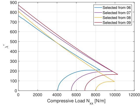
Fig. 10 Combined flutter-buckling diagrams for selected configurations from O6, O7, O8 and O9.
