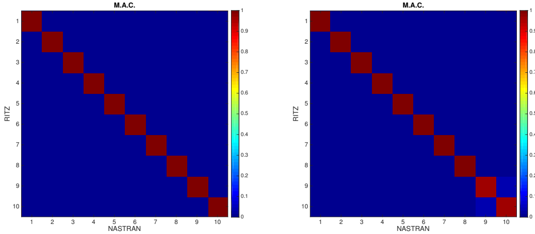
Fig. 2 Mode Assurance Criteria for: (a) configuration A; (b) configuration B
