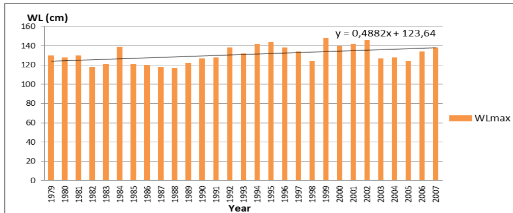
Figure 13: Trend of highest water level in the period 1979 to 2007 at Vungtau station.
