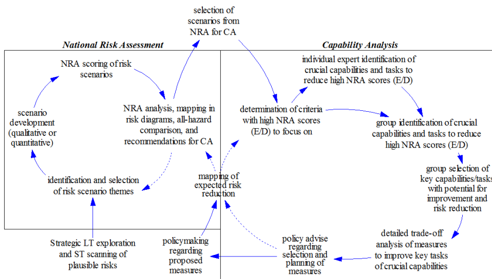
Figure 1: Iterative process of the state of the art Integrated Risk Assessment and Capability Analysis not under deep uncertainty
