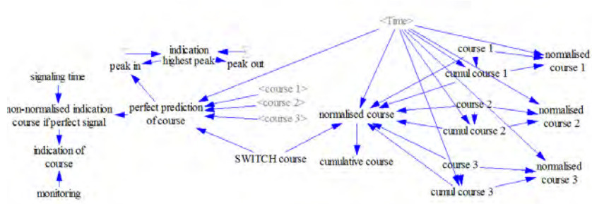
(a) structures to simulate multiple evolutions over time
