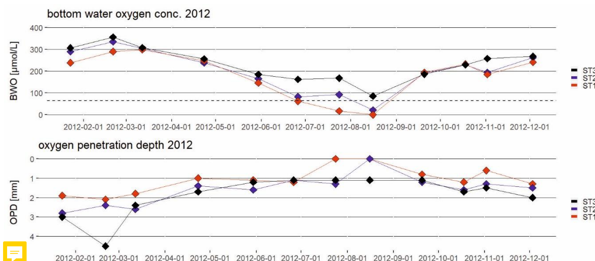
Figure 6. A: BWO concentration for stations ST1 (34 m), ST2 (23 m) and ST3 (17 m) with indicated sampling dates in 2012. The dashed line indicates the threshold for hypoxic conditions (63 µmol/L). B: Oxygen Penetration Depth for ST1, ST2 and ST3 measured from sediment cores sampled on the same dates in 2012 as water column parameters. Data from Hagens et al. (2015) and Seitaj et al. (2017).
