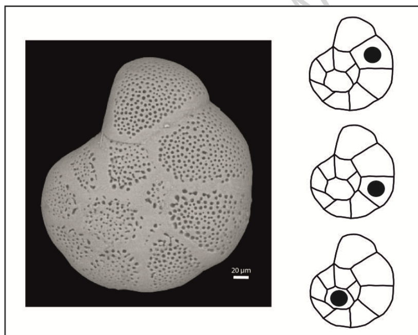
Fig 2. Left: SEM image of A. tepida specimen (presumably phylotype T6 based on morphological distinction as shown by Richirt et al., 2019) from Lake Grevelingen (image taken at SCIAM, University of Angers). Right: Sketches to show location of LA-ICP-MS spot analysis on penultimate chamber (top), antepenultimate chamber (middle) and central part of test (bottom).
