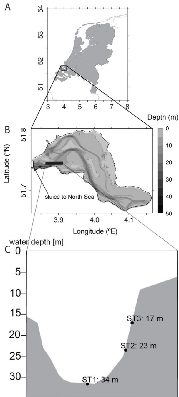
Figure 1. Location map of Lake Grevelingen and the three sampling stations in this study. A: map of the Netherlands. B: bathymetry of Lake Grevelingen, the sluice giving access to the North Sea is situated at the most western end of the lake. C: depth cross-section of the Den Osse basin (W-E) with locations of stations ST1, ST2 and ST3. Modified from Hagens et al. (2015).
