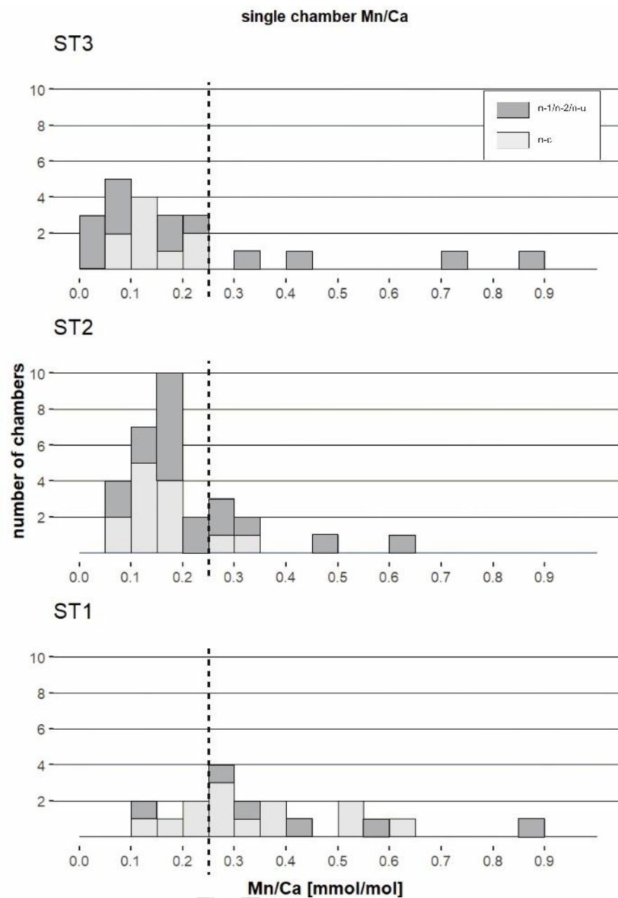
Figure 3. Histograms for all Mn/Ca measurements (individual chambers in dark grey, and central part of the test in light grey) for the three stations (bin width= 0.05 mmol/mol). Kruskal-Wallis test p value :< 0.001 (for data of n-1/n-2/n-u and n-c combined). Wilcoxon-Mann-Whitney post-hoc test p values: < 0.001 (ST1 vs ST2), < 0.001 (ST1 vs ST3) and 0.220 (ST2 vs ST3). Dashed line indicating 0.25 mmol/mol (see section 3 for explanation).
