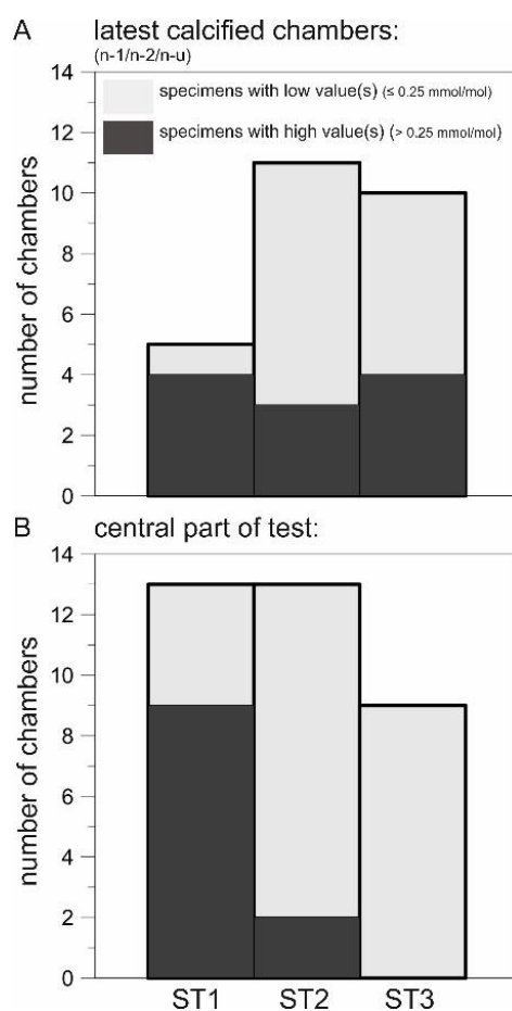
Figure 5. Specimens with high Mn/Ca ratios in comparison to total number of specimens measured for each station (data in Tab. 4). A: Latest calcified chambers (n-1, n-2, n-u). B: Central part of test.
