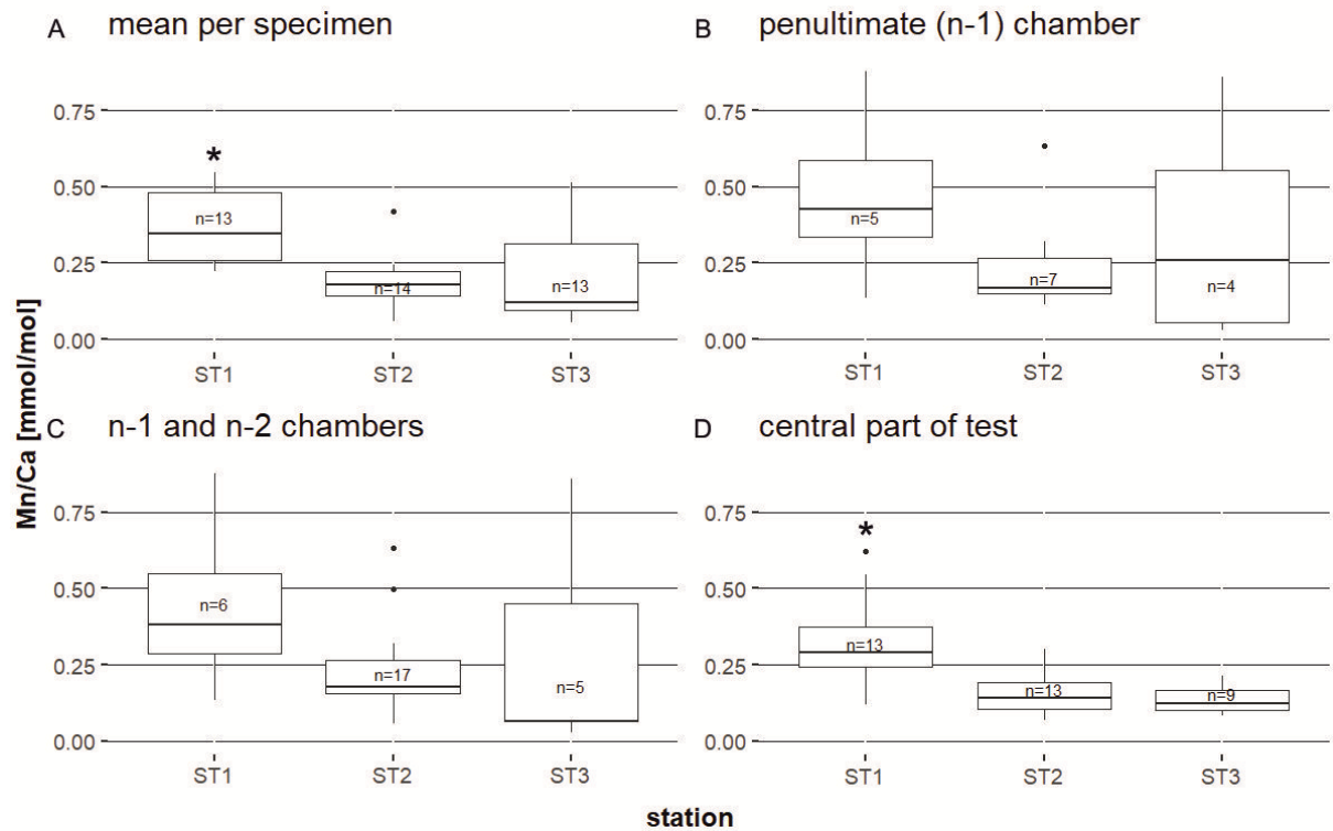
Figure 4. Boxplots of Mn/Ca ratios for all specimens of A. tepida from stations ST1 (34 m), ST2 (23 m) and ST3 (17 m) sampled in July 2012. A: mean per specimen (n indicates number of specimens). B: penultimate chamber (n indicates number of single chamber ablations, also in C and D). C: n-1 and n-2. D: central part of test. Data for n-u (n = 8) not represented. Significant differences for ST1 compared to ST2 and ST3 are indicated by *.
