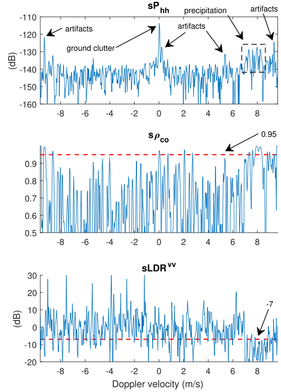
Fig. 4. Observable spectra of Range bin 468 (e.g., 14 km). (a) Spectral power sP_{hh} . (b) Spectral copolar correlation coefficient s\rho_{co} . (c) sLDR^{vv} .
