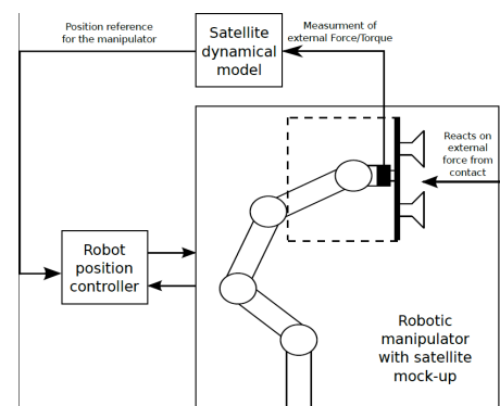
Figure 2: Conceptual control diagram of the TRH Free-floating Satellite dynamics test-bed for hardware-in-the-loop docking experiments.
