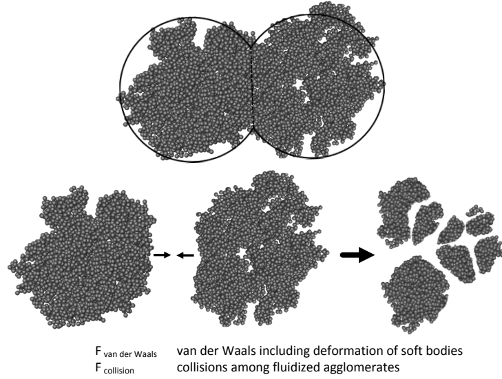
Figure 3: Schematic of the force balance on fluidized agglomerates. Van der Waals is the main force holding the agglomerates together, counteracted by the dominant separation force arising from collisions.
