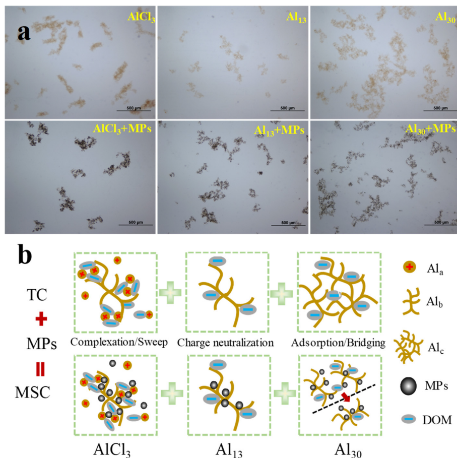
Fig. 6. Coagulation (a) floc images and (b) concept models of \text{AlCl}_3 , \text{Al}_{13} and \text{Al}_{30} in the TC and MSC process.
