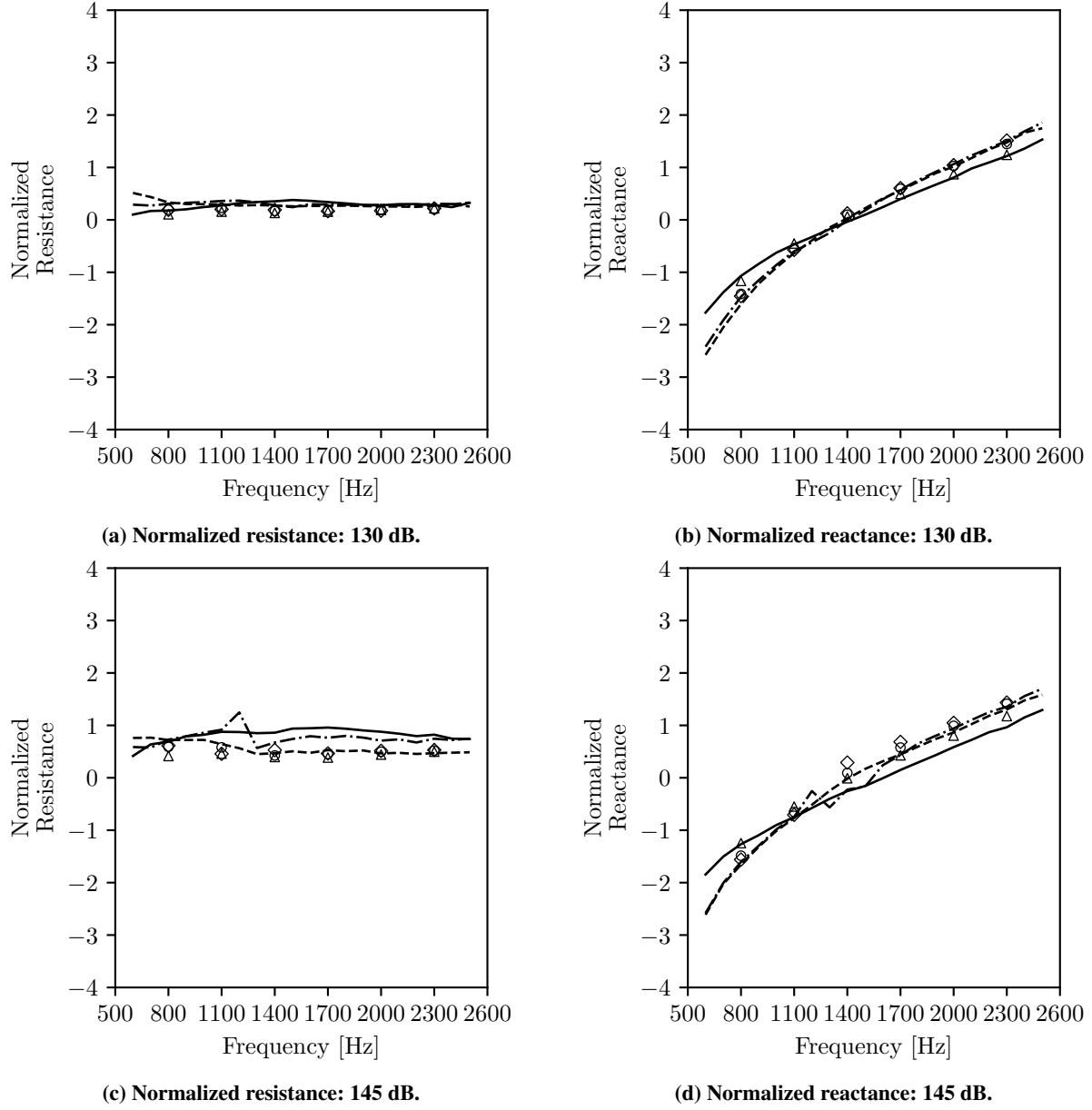
Fig. 6 Normalized impedance for the no-flow case as a function of the incident acoustic wave frequency: (—) experimental [in-situ]; (- -) experimental [MM]; (- · -) experimental [KT]; ( \Delta ) numerical [in-situ]; ( \circ ) numerical [MM]; ( \diamond ) numerical [KT].
