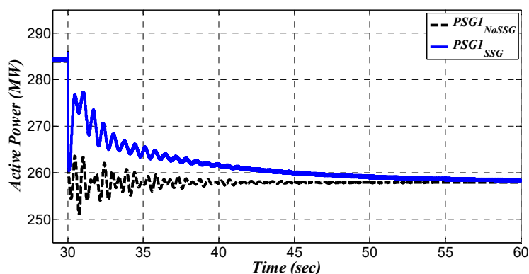
Figure 20. Active power of generation unit in bus (1).
