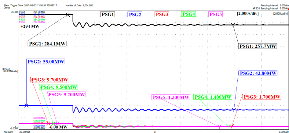
Figure 35. Oscillations in generated active powers—base case.
