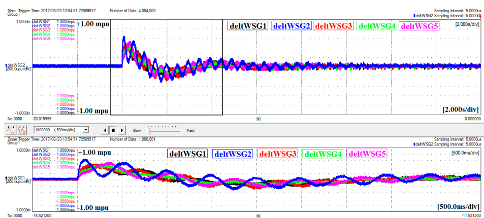
Figure 33. Frequency deviation of generation units—base case.
