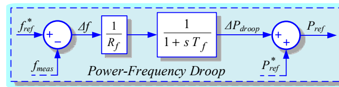
Figure 5. Participation of RSSG-SPC in primary frequency control.
