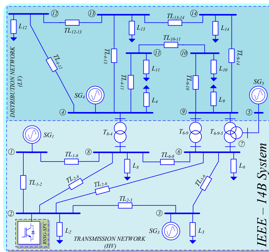
Figure 12. RSSG-SPC in IEEE 14-bus test system.
