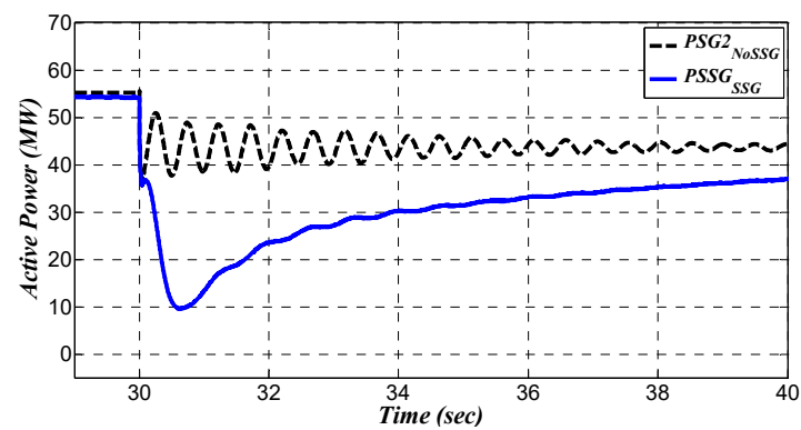
Figure 22. Absorption of damped active power by RSSG-SPC in bus (2).
