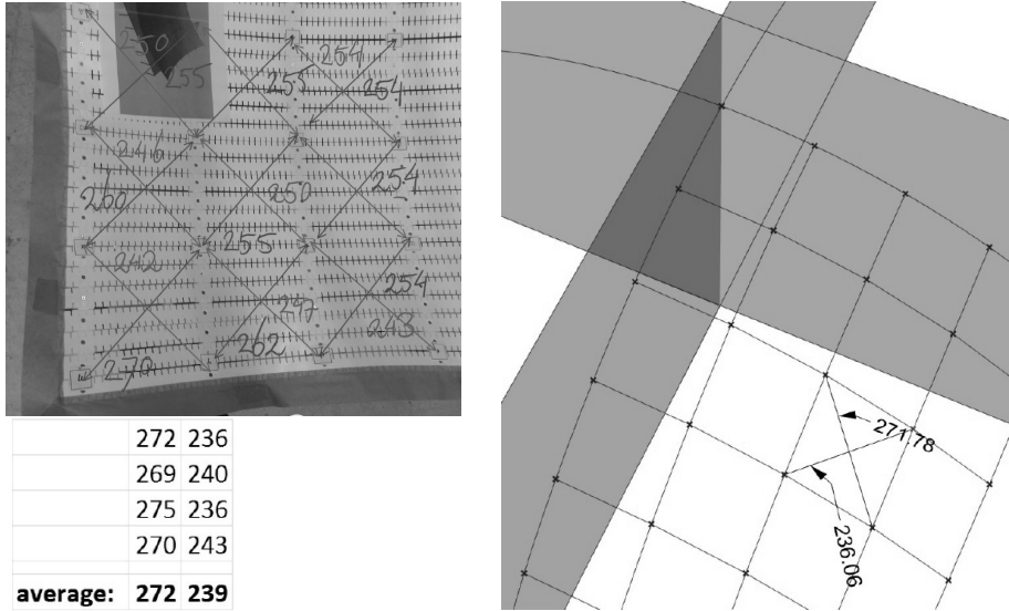
Figure 11: The shear angle in the Rhino-GH model compared to that in the prototype, R = 1200 mm. Fairly good correspondence (error below 2%) is found between the values calculated using the model and the average values measured over four mould corners of the prototype set-up.
