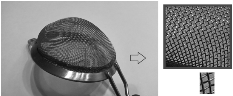
Figure 6: A kitchen sieve clearly shows the principle of shear-deformation: a flat steel mesh can be formed into a double-curved surface, by allowing shear angles between the woven wires of the sieve. Although it cannot be completely ruled out that also stretching of the wires has occurred, shear deformation will result in the required shape with limited force.
