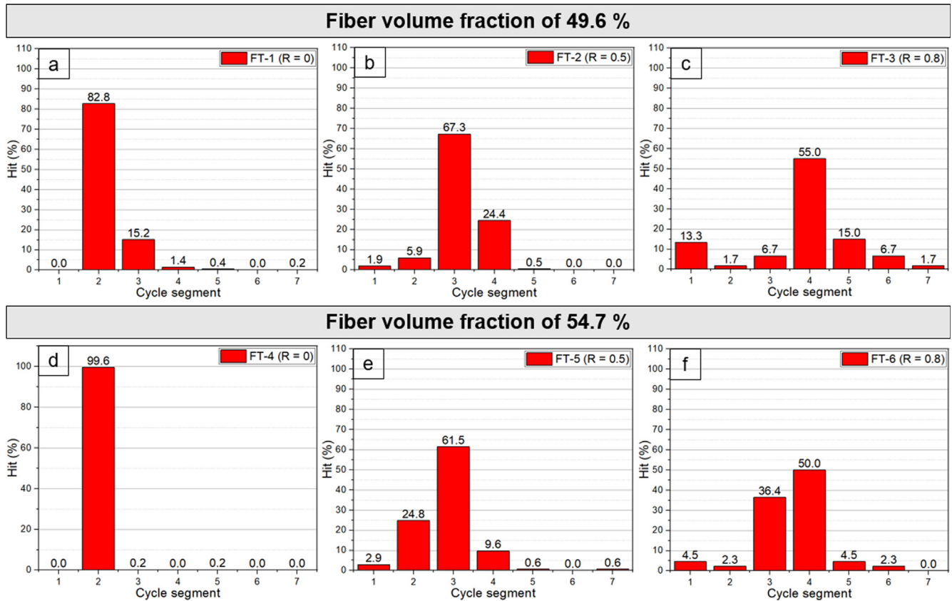
Fig. 7. Distribution of the first hits in each loading cycle during the first five hundred fatigue cycles (the hits detected in section 1 of the specimens FT-1 and FT-4 were not considered as damage onset). (For interpretation of the references to colour in this figure legend, the reader is referred to the web version of this article.)
