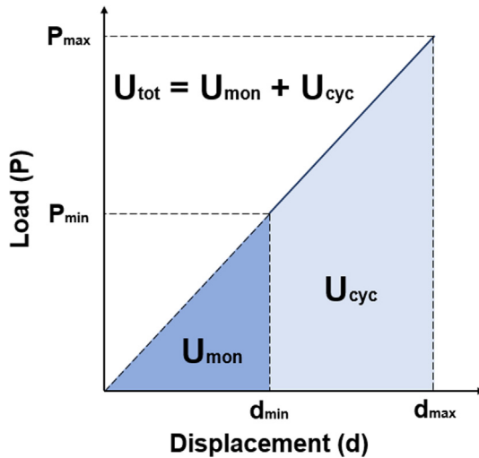
Fig. 5. Schematic diagram of load ( P ) versus displacement ( d ) with the definitions of U , U_{\text{mon}} and U_{\text{cyc}} . (For interpretation of the references to colour in this figure legend, the reader is referred to the web version of this article.)
