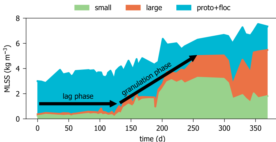
Figure 5.2: Typical startup of an aerobic granular sludge reactor from flocs, showing an initial lag phase with slow improvement of the sludge morphology, followed by the granulation phase, where granules appear in the reactor. The colours indicate the size of the biomass aggregates, showing proto-granules and flocs ( <200\ \mu\text{m} ), small granules ( >200\ \mu\text{m} ) and large granules ( >1000\ \mu\text{m} ). Data derived from the Nereda ® reactor in Utrecht, the Netherlands.
