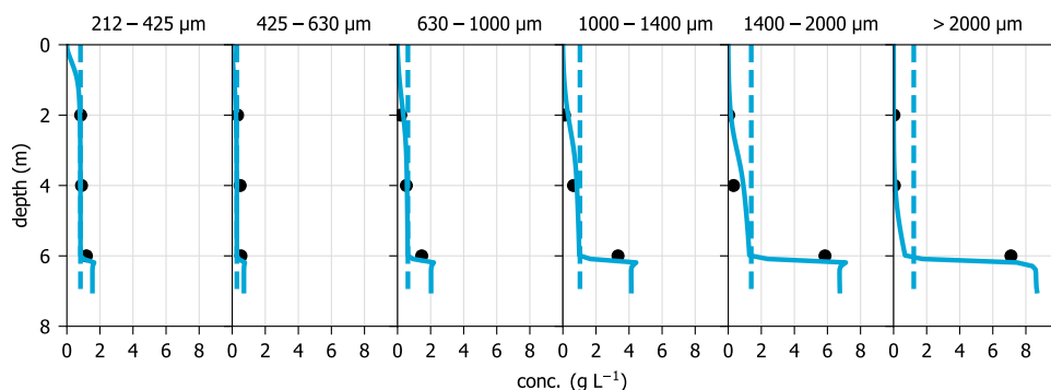
Figure 3.8: Settling of 6 classes of granules in a full-scale Nereda® reactor in Utrecht after 0 minutes and after 15 minutes; model results (dashed line: 0 minutes, solid line: 15 minutes) and measurements (dots).
