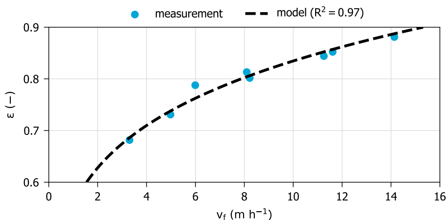
Figure 3.7: Bed expansion experiment with sieved granules (1 to 2 mm) from the Prototype Nereda® Utrecht; data points were used to fit the extrapolated fluidizing velocity and the expansion index according to equation 3.9.
