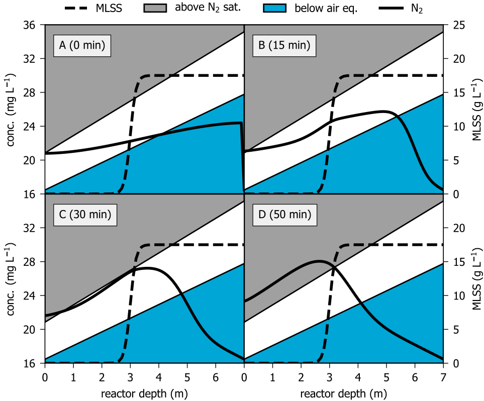
Figure 2.6: effect of feeding after a stripping phase on the dissolved nitrogen gas concentration from the start (A), after 15 minutes (B), after 30 minutes (C) and after 50 minutes (D). T = 13.5^{\circ}\text{C} , r = 0.25 \text{ mg g}^{-1} \text{ h}^{-1} . Black solid line: the actual \text{N}_2 concentration, black dashed line: biomass concentration, grey area: \text{N}_2 concentration above saturation, blue area: \text{N}_2 concentration below equilibrium with air, boundary between grey area and white area: \text{N}_2 concentration at equilibrium with pure nitrogen gas at ambient water pressure, boundary between blue area and white area: \text{N}_2 concentration at equilibrium with air at ambient water pressure.
