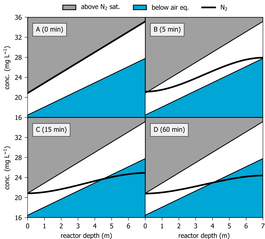
Figure 2.5: Stripping of N_2 gas from fully saturated situation (A) and after 5 minutes (B), 15 minutes (C) and 60 minutes of stripping (D) at 13.5 °C. Black solid line: the actual N_2 concentration, grey area: N_2 concentration above saturation, blue area: N_2 concentration below equilibrium with air, boundary between grey area and white area: N_2 concentration at equilibrium with pure nitrogen gas at ambient water pressure, boundary between blue area and white area: N_2 concentration at equilibrium with air at ambient water pressure.
