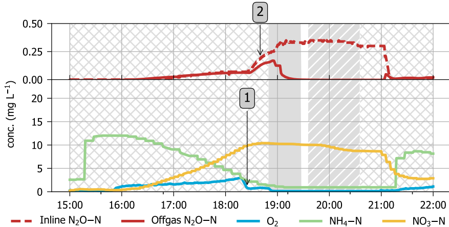
Figure 4.13: Increase of the nitrous oxide production [marker 2] when the oxygen concentration dropped to a value below 1 \text{ mg L}^{-1} [marker 1]. The grey diagonal striped area indicates the feeding phase, the grey diamond grid shows the reaction phase and the grey solid area shows the settling phase.
