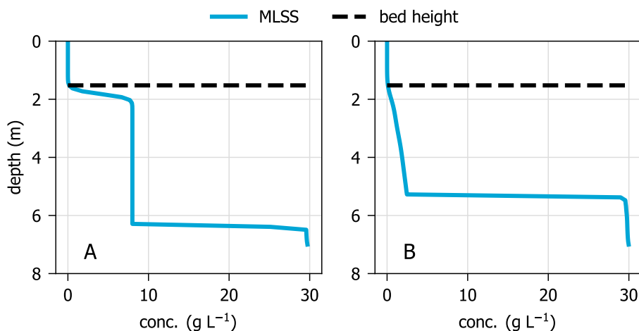
Figure 3.10: Comparison of the settling of a uniformly sized (A) and a disperse (B) granular sludge bed both after 30 minutes of settling. Left: uniform bed with 8\text{ g L}^{-1} granules of 700\text{ }\mu\text{m} , right: disperse bed with 8\text{ g L}^{-1} (sizes: 318 , 527 , 815 , 1200 , 1700 and 3000\text{ }\mu\text{m} ; concentration: 1 , 1 , 1 , 1 , 2 and 2\text{ g L}^{-1} ).
