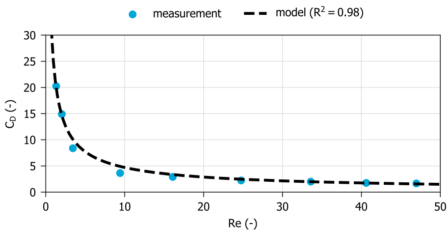
Figure 3.4: Drag coefficient of individual granules from the full-scale Nereda ® plant in Garmerwolde; the data points were used to fit the a and b parameters of equation 3.7.
