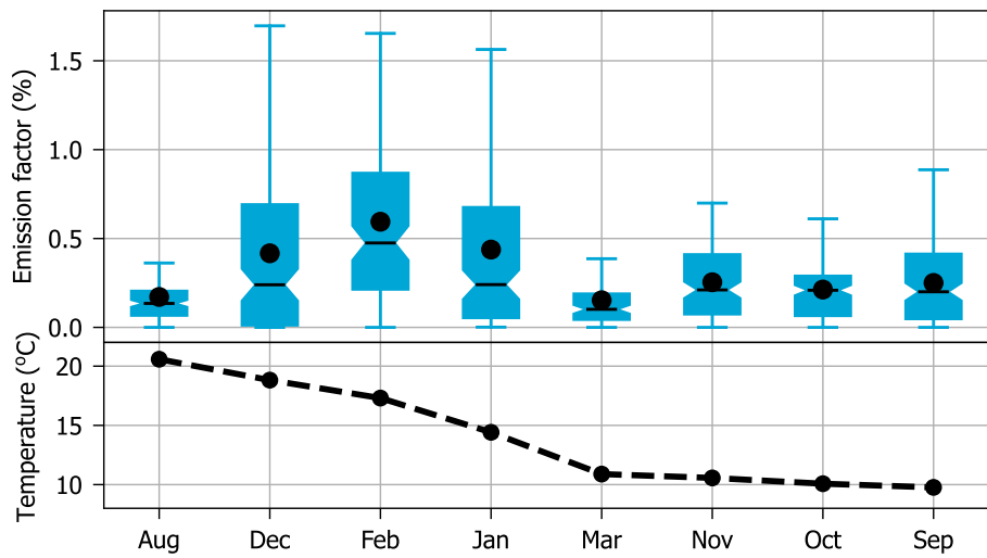
Figure 4.6: Top: boxplot of the monthly averaged nitrous oxide emission factor (the box extends from 25 % to 75 % values, the black line shows the median value, the black dot shows the average value and the whiskers extend the range of the data); bottom: monthly average temperature profile.
