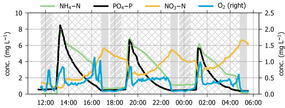
Figure 4.5: Concentration profiles of ammonium (green), nitrate (orange), phosphate (black) and oxygen (blue) for three typical consecutive batches. The grey diagonal striped area indicates the feeding phase, the grey diamond grid shows the reaction phase and the grey solid area shows the settling phase.
