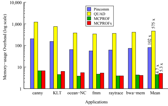
Fig. 10: Comparison of Memory-usage overhead.
