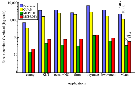
Fig. 9: Comparison of execution-time overhead.
