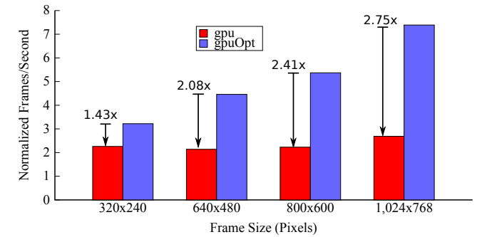
Fig. 8: Normalized Frames per seconds achieved by the GPU and data-communication optimized GPU implementation.
