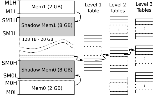
Fig. 4: Hybrid Shadow Memory Scheme Utilized by MCPROF. Most Frequently Accessed Regions of Memory (Mem0 and Mem1) use Direct Mapping. Rest of the Memory Map is Shadowed by 3-Level Table Lookup.
