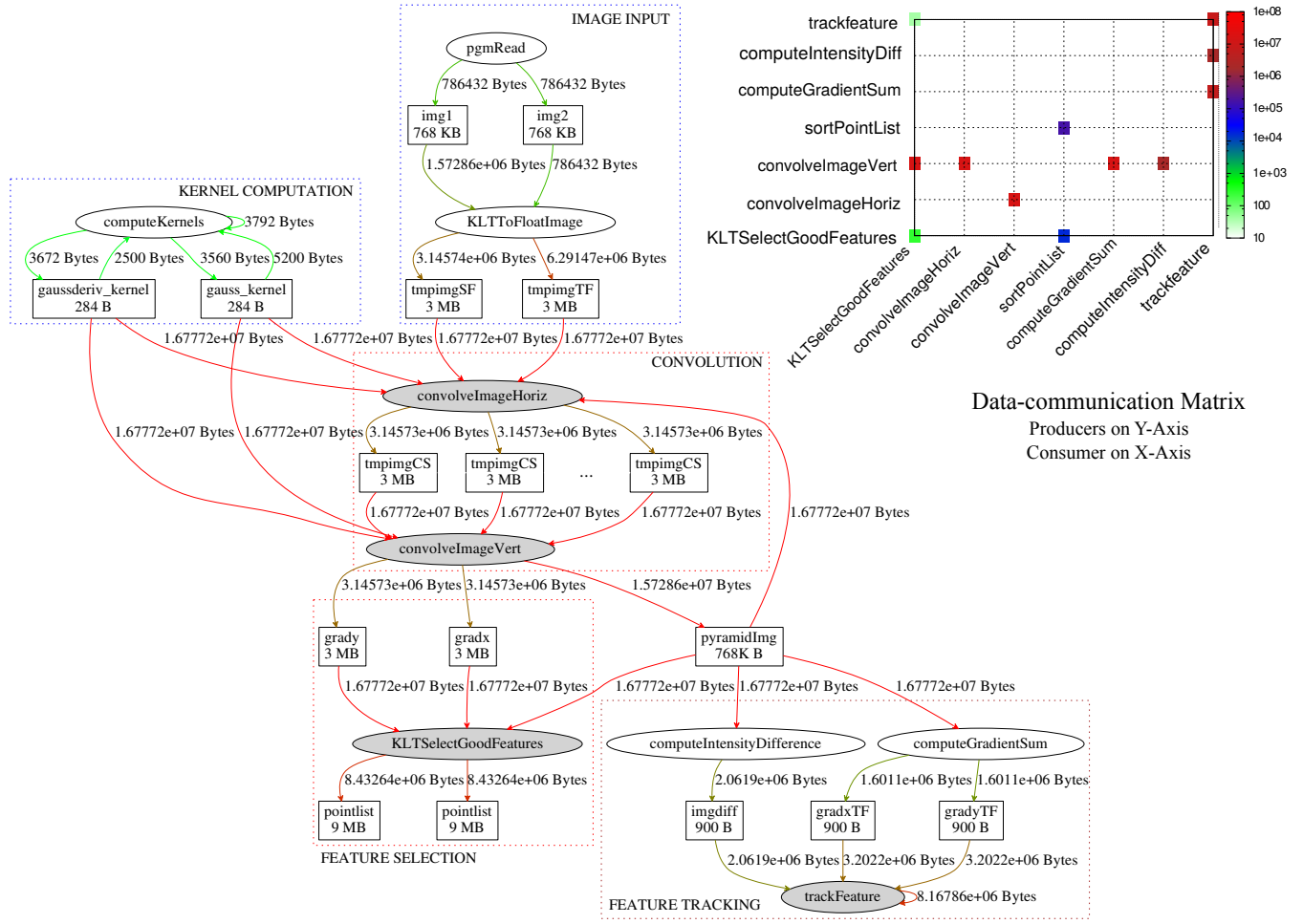
Fig. 7: KLT Communication Matrix (top right) and communication graph generated by MCPROF. Functions (ovals), compute-intensive functions (Grey ovals) and the objects(rectangles) involved in the communication are also shown.
