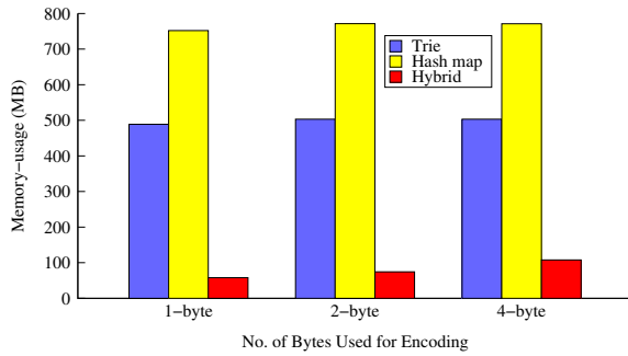
Fig. 14: Memory-usage Comparison of three Data-structures with Varying Number of Encoding Bytes.
