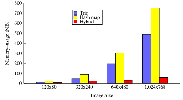
Fig. 12: Memory-usage Comparison of Data-structure access only.
