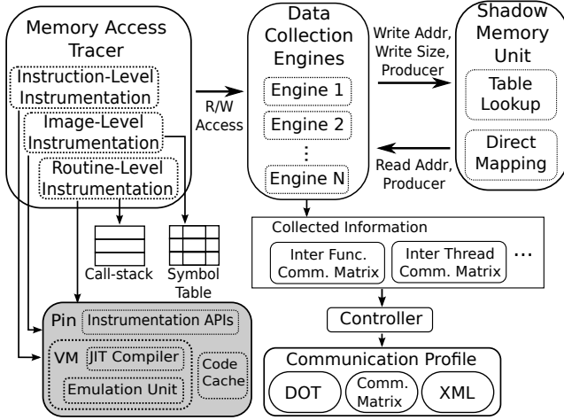
Fig. 2: Internal organization of MCPROF.
