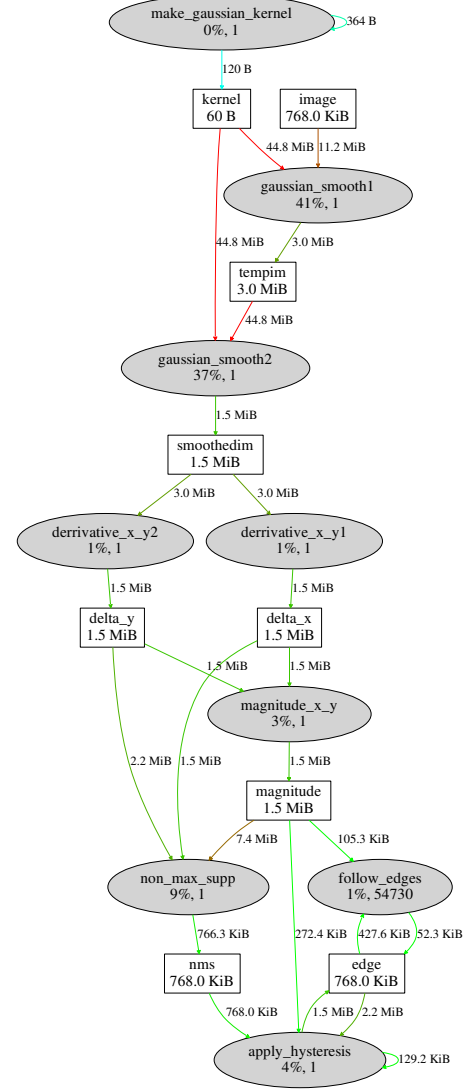
Fig. 5: Data-flow graph of Canny application generated by MCPROF.
