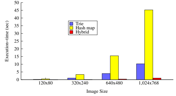
Fig. 11: Execution-time Comparison of Data-structure access only.
