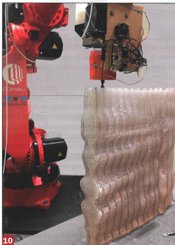
3D printing of part of the prototype using a robotic arm with a custom-made FDM extruder and print head
