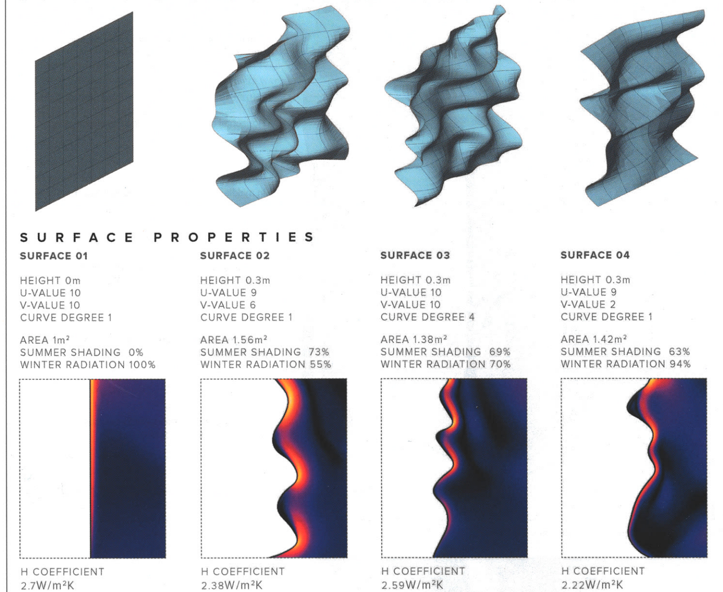
Results of simulations with Comsol showing how the air flows along a vertical surface in case of free convection for different surface geometries, and the resulting boundary heat transfer coefficient ( h ) and surface area ( A ). h \cdot A is a measure for the total convective heat transfer. White represents the material of the wall, colours represent the velocity of the air from low speed (purple) towards higher speed (yellow) [14]
