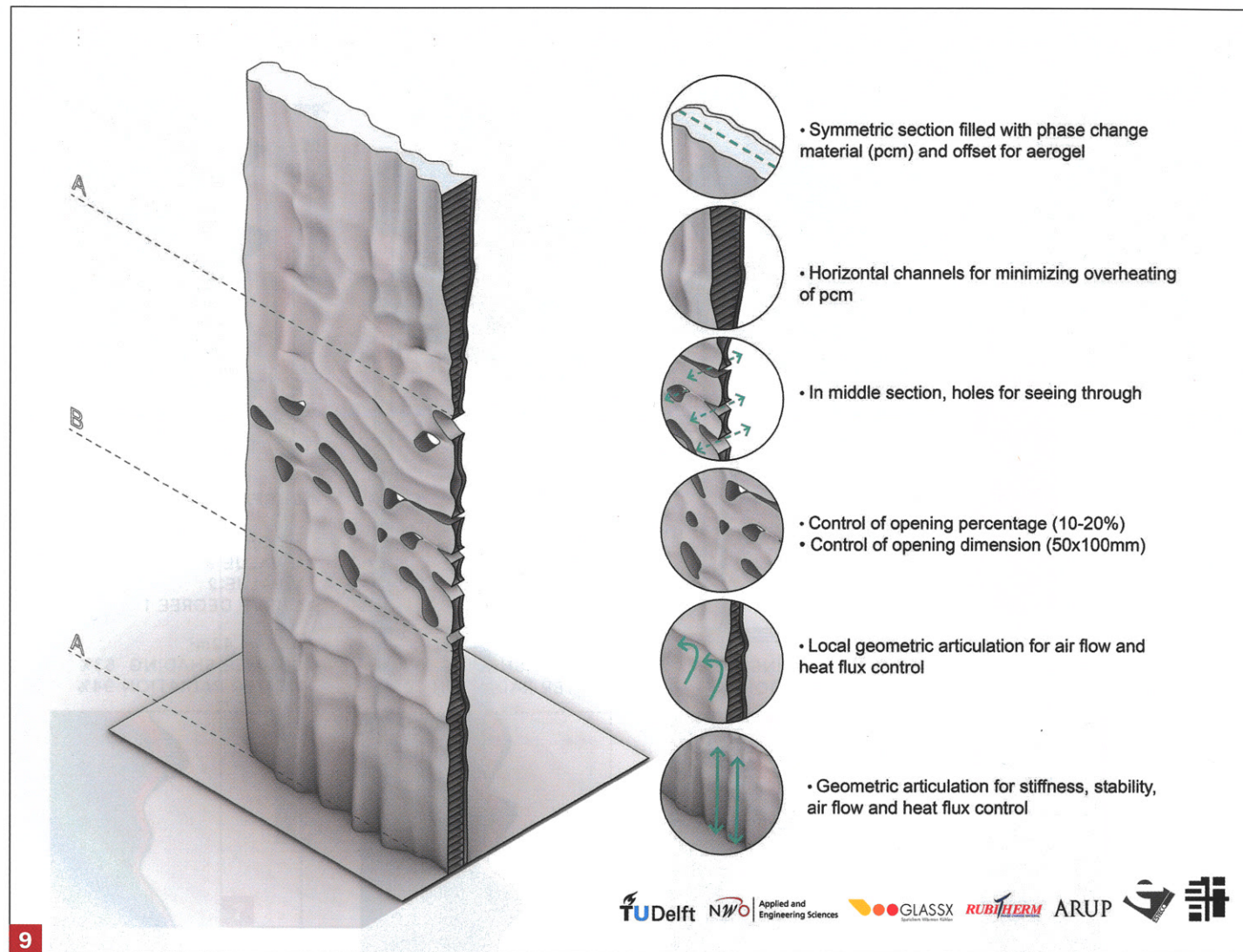
Integrated design concept of the prototype
