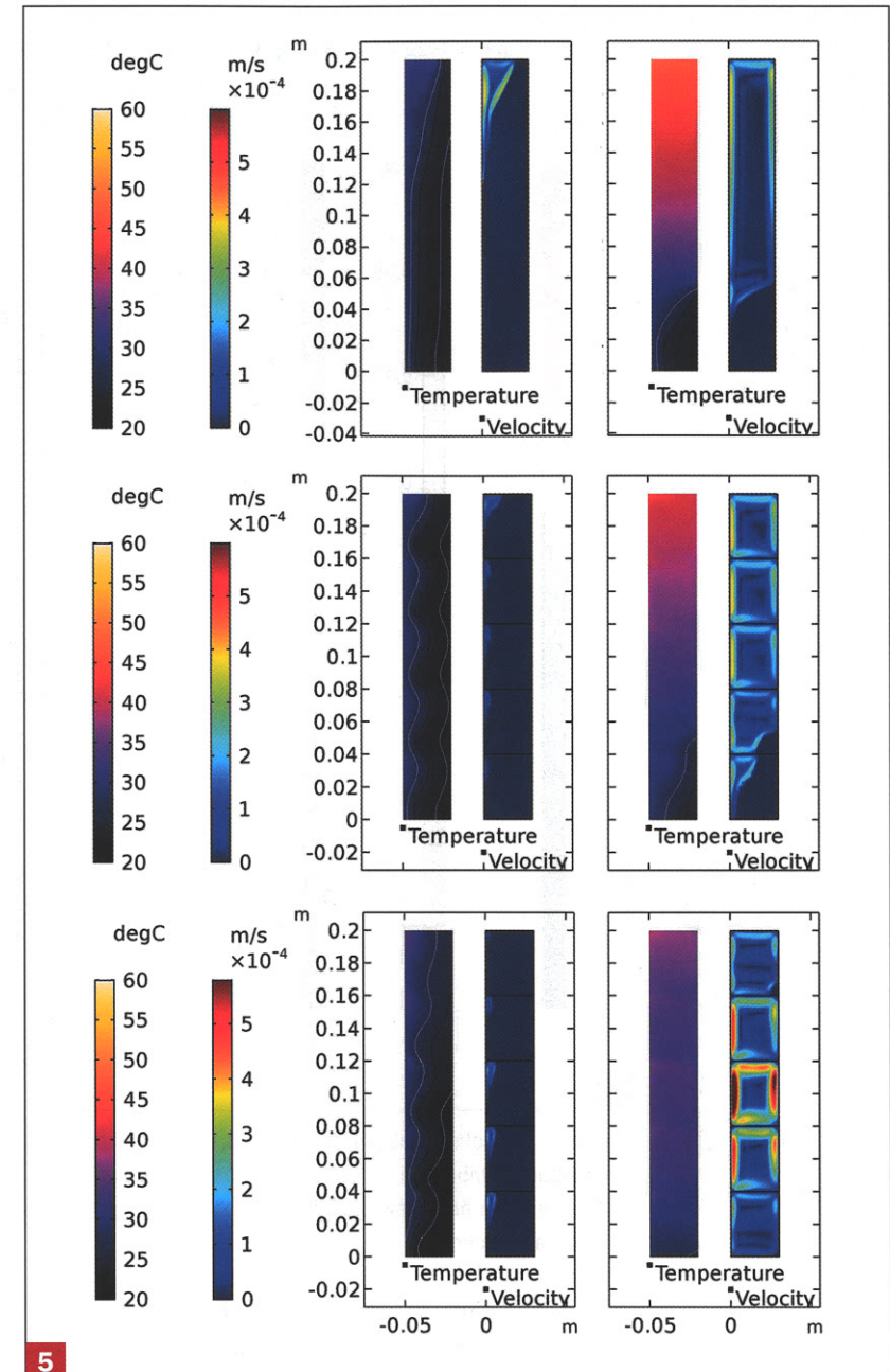
Results of the simulations with Comsol showing the temperature and velocity distribution of the PCM inside the Trombe wall after 4 hours (left column) and 8 hours (right column) of exposure to solar radiation of 300 W/m 2 from the left side. The image at the top presents a full column of PCM with a phase transition around 25°C of 3 cm thick and 20 cm high; the image at the middle shows the same column of PCM but now segmented into smaller pieces of 4 cm high; the image at the bottom shows the segmented PCM column with different PCM phase change temperatures (from bottom to top: 23, 24, 25, 27, 29°C) [12]
