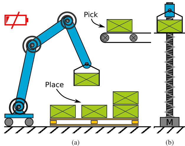
Fig. 1: Plugless robot arm. (a) Explains the idea; the robot performs a pick and place task where the pick position is higher than the place position. With aid of (nonlinear) springs, as illustrated on the joints, the gravitational energy of the package can be recovered to power the robot. (b) Shows the simulation model, consisting of a single degree of freedom robot including a motor and transmission model.
